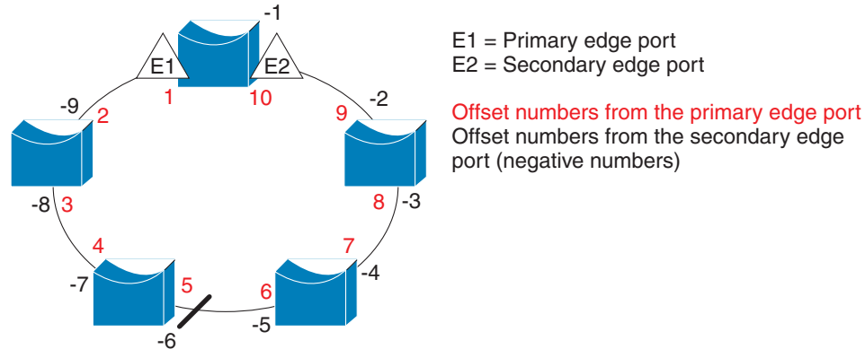
Figure 18-3 Neighbor Offset Numbers in a Segment
