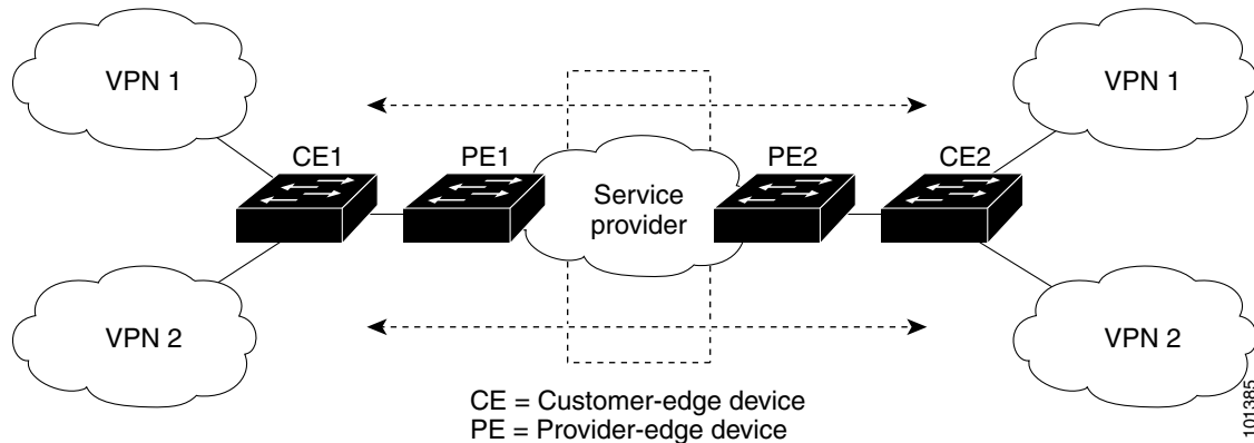
Figure 36-6 Switches Acting as Multiple Virtual CEs
