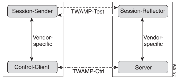
Figure 39-4 TWAMP Architecture
