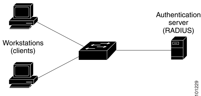
Figure 8-1 IEEE 802.1x Device Roles
