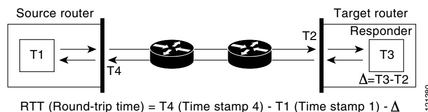
Figure 39-2 Cisco IOS IP SLAs Responder Time Stamping
