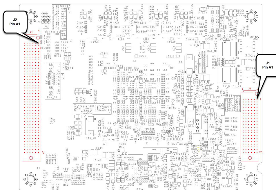
Figure 1: Interface Connectors Bottom Side View
