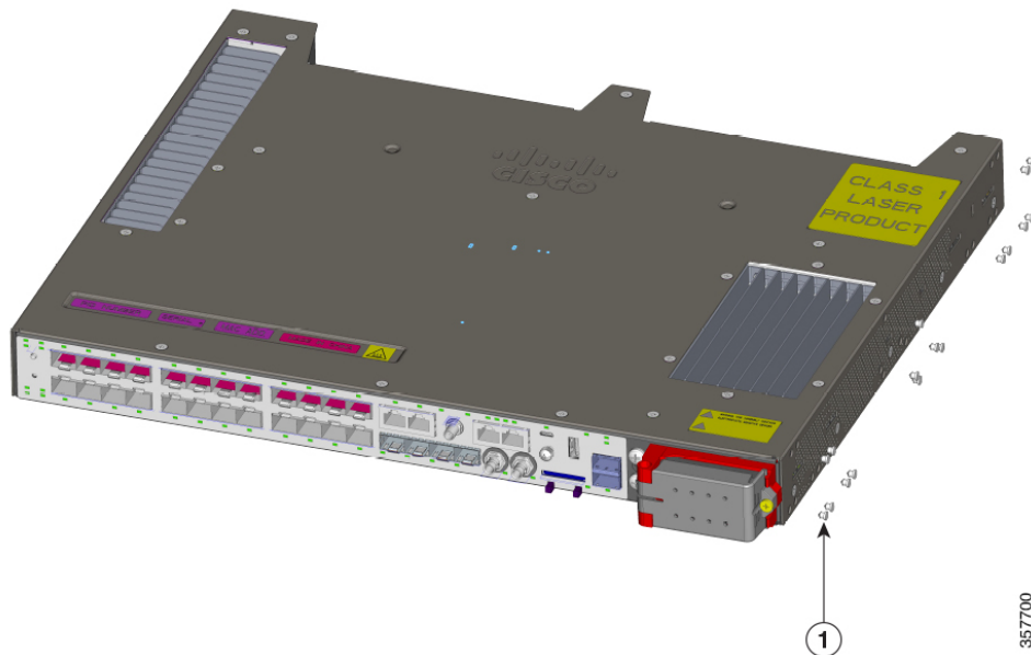
Figure 5: Switch Hole Locations
