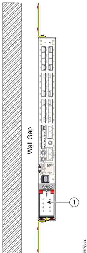
Figure 11: Wall-Mount Clearance
