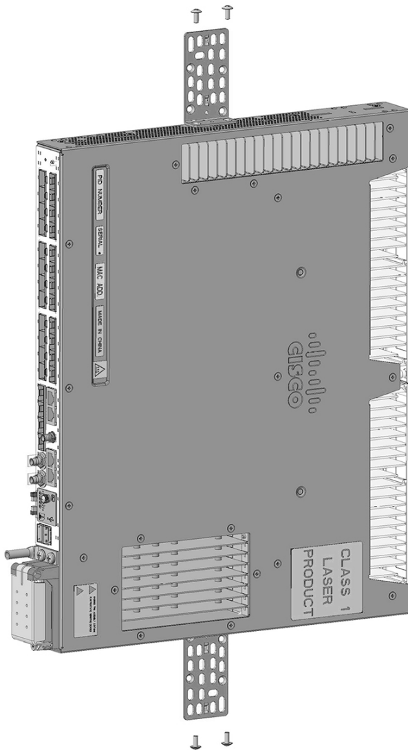
Figure 12: Attaching the Brackets for Wall Mounting
