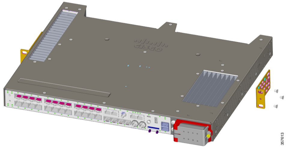
Figure 2: Attaching Brackets: Middle Mounting
