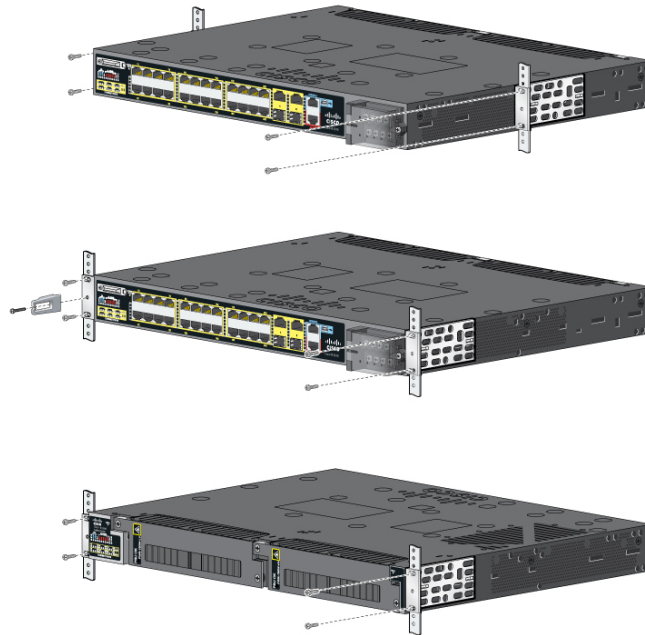
Figure 9: Rack-Mounting the Switch
