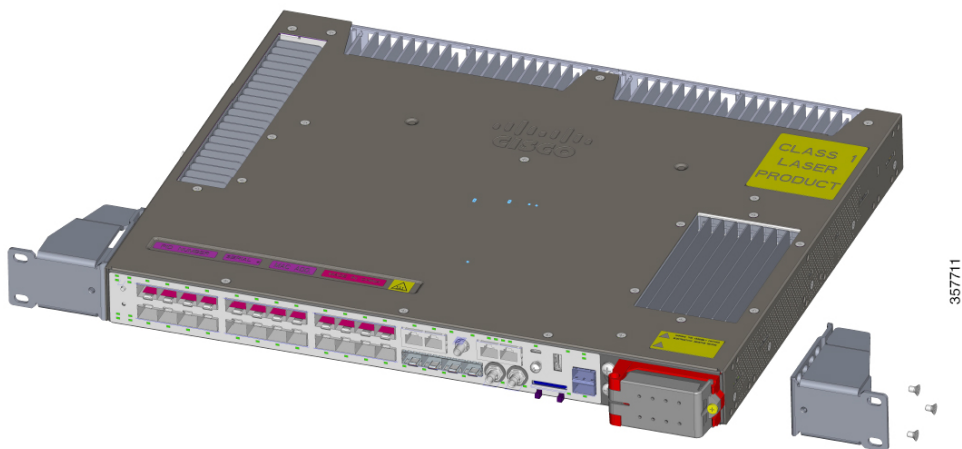
Figure 6: Attaching Brackets for 23-inch Racks (Front Mounting)
