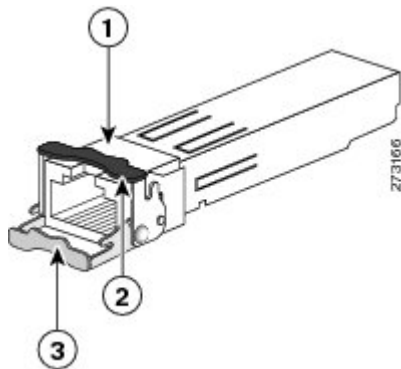
Figure 14: 1000BASE-T SFP Transceiver
