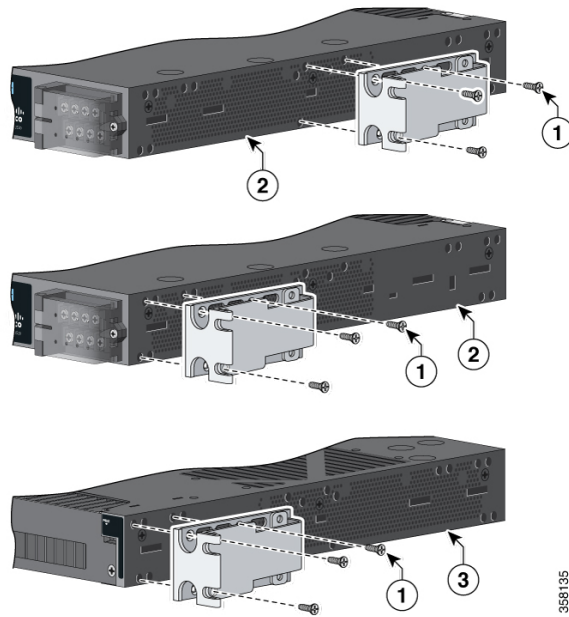
Figure 8: Attaching Brackets (RM-RGD-ETSI=) for ETSI Racks
