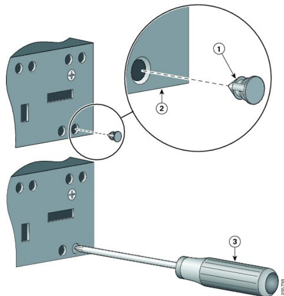
Figure 4: Inserting a Rubber Plug
