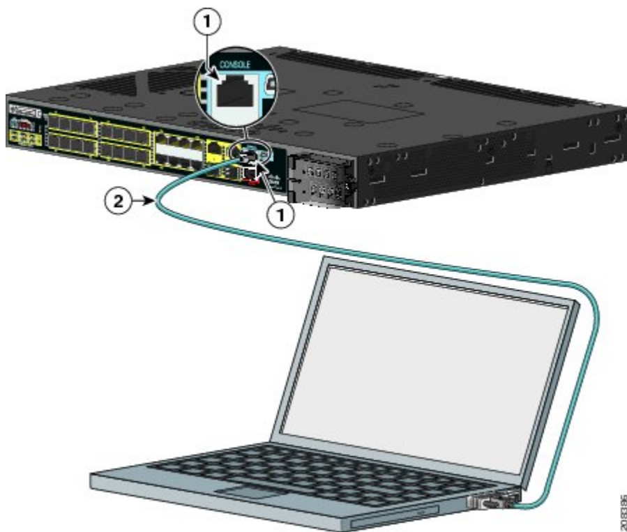
Figure 1: Connecting the Console Cable
