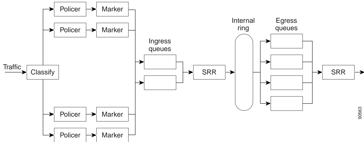
Figure 37-6 Ingress and Egress Queue Location
