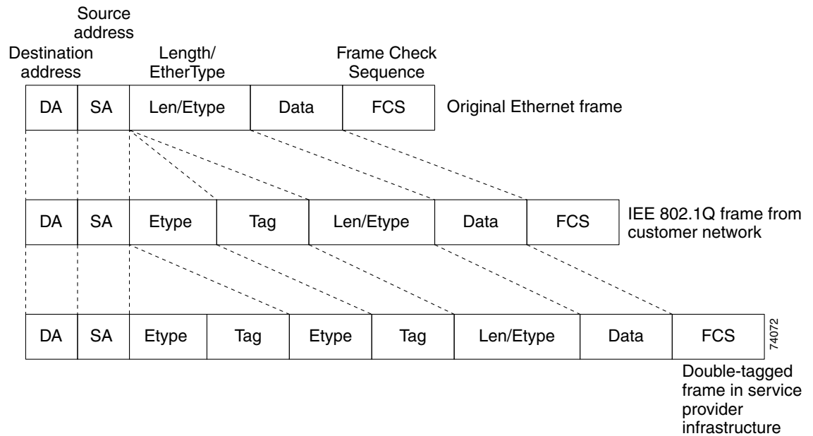
Figure 20-2 Original (Normal), IEEE 802.1Q, and Double-Tagged Ethernet Packet Formats
