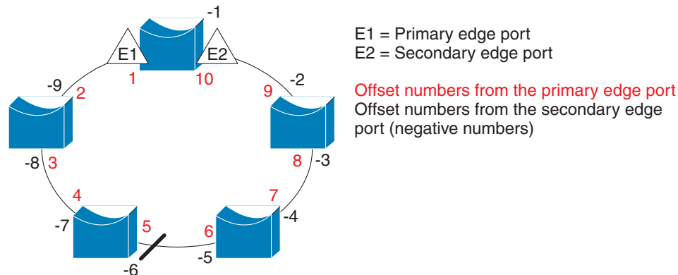
Figure 20-4 Neighbor Offset Numbers in a Segment
