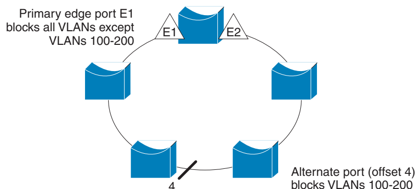
Figure 20-5 Example of VLAN Blocking
