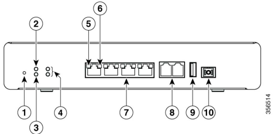
Figure 6: Front Panel of CGP-ONT-4PVC
