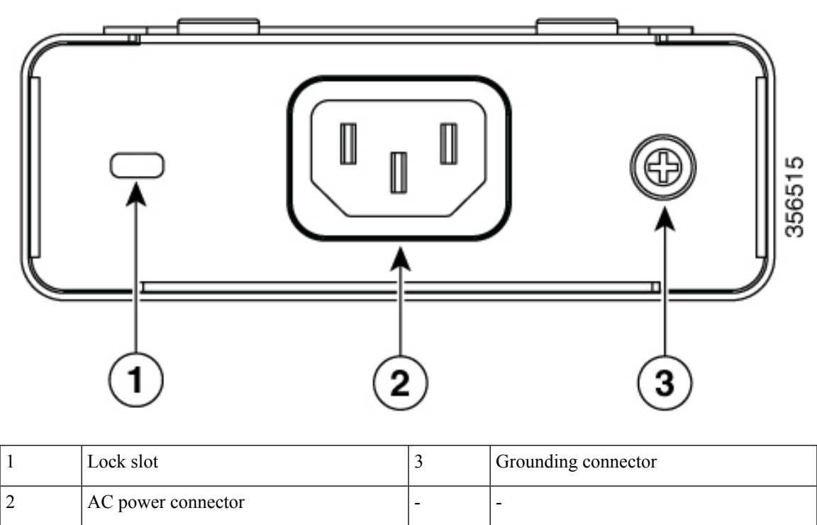
Figure 9: Rear Panel of CGP-ONT-4PVC
