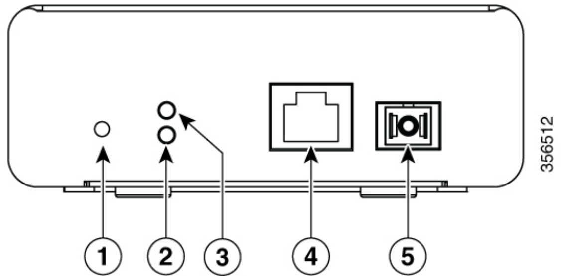
Figure 5: Front panel of CGP-ONT-1P
