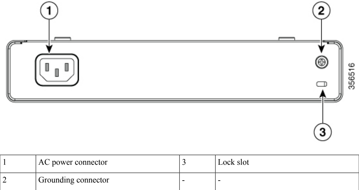
Figure 9: Rear Panel of CGP-ONT-4PVC
