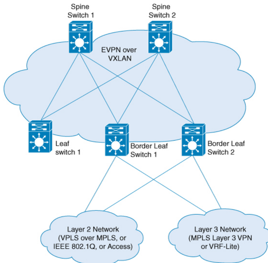
Figure 32: EVPN VXLAN External Connectivity Through a Border Leaf Switch
