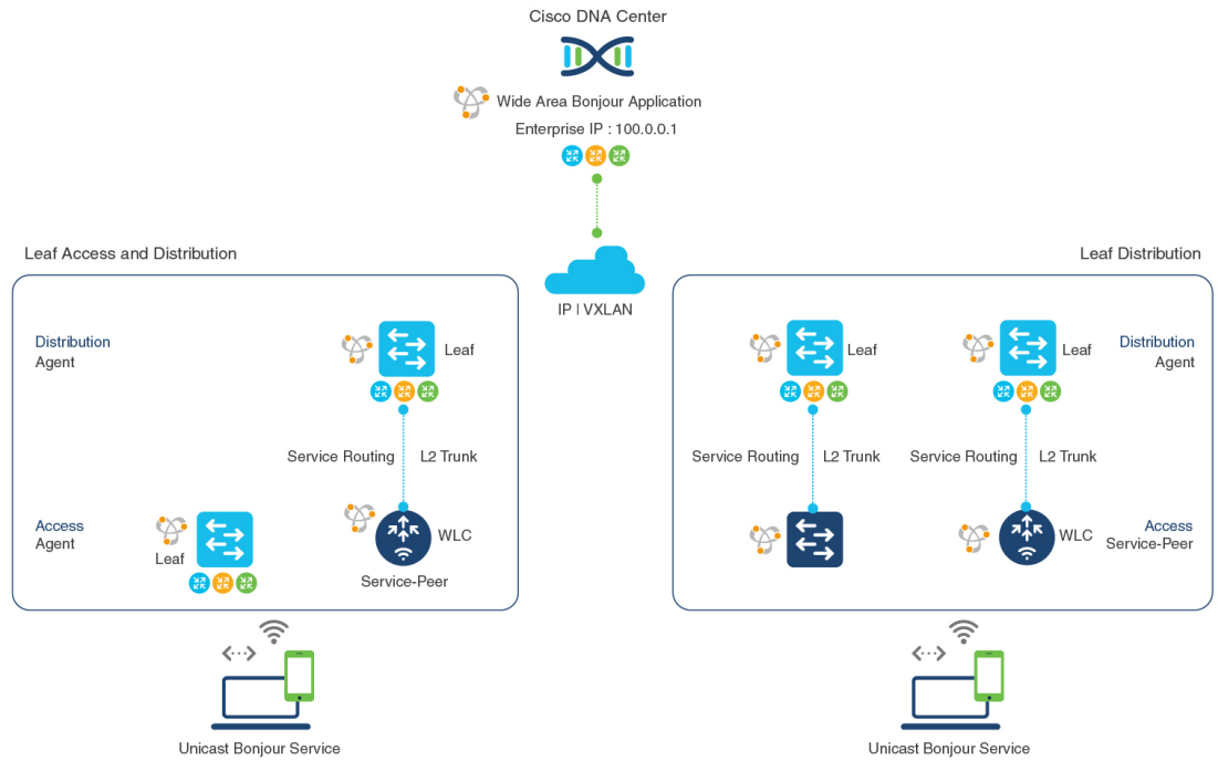
Figure 80: Deployment Model for Wide Area Bonjour over BGP EVPN VXLAN
