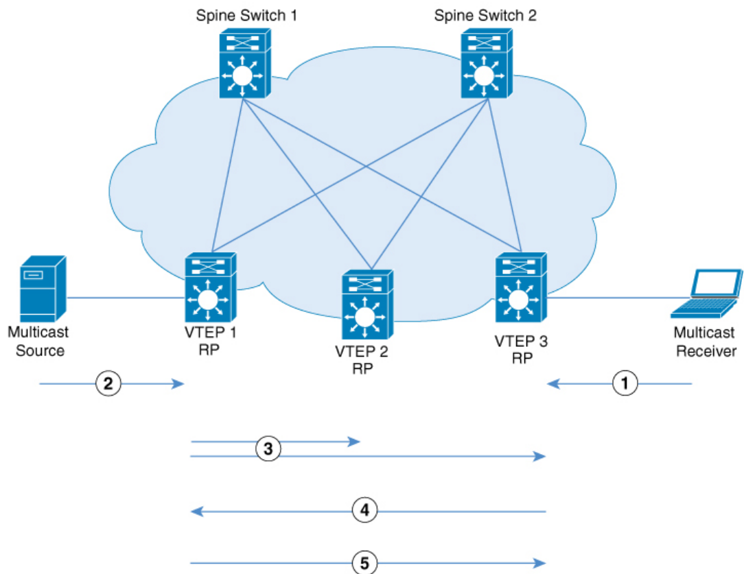
Figure 25: PIM Sparse Mode with Anycast RP
