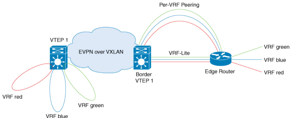
Figure 34: Layer 3 External Connectivity with VRF-Lite
