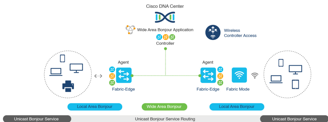
Figure 70: Cisco SD-Access Wired and Wireless Network Design
