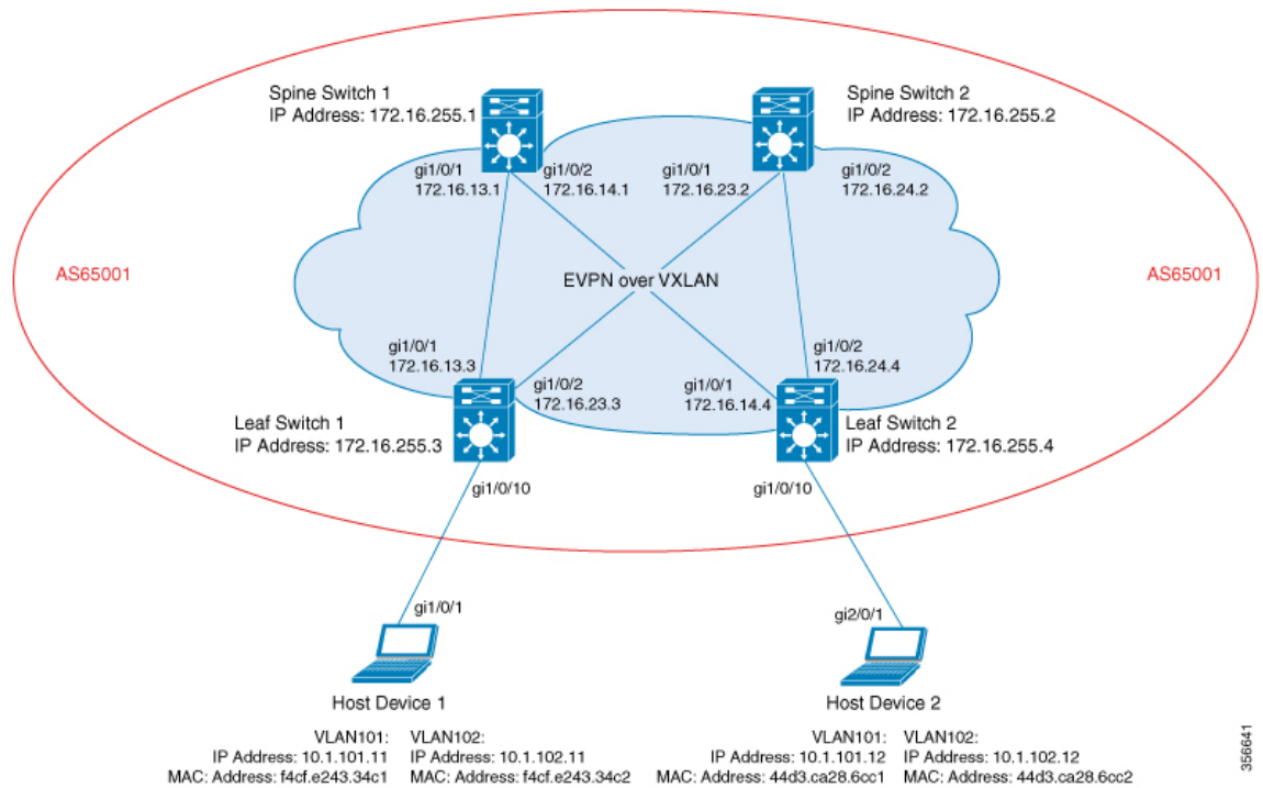
Figure 14: BGP EVPN VXLAN Fabric with the Spine Switches and Leaf Switches in the Same Autonomous System
