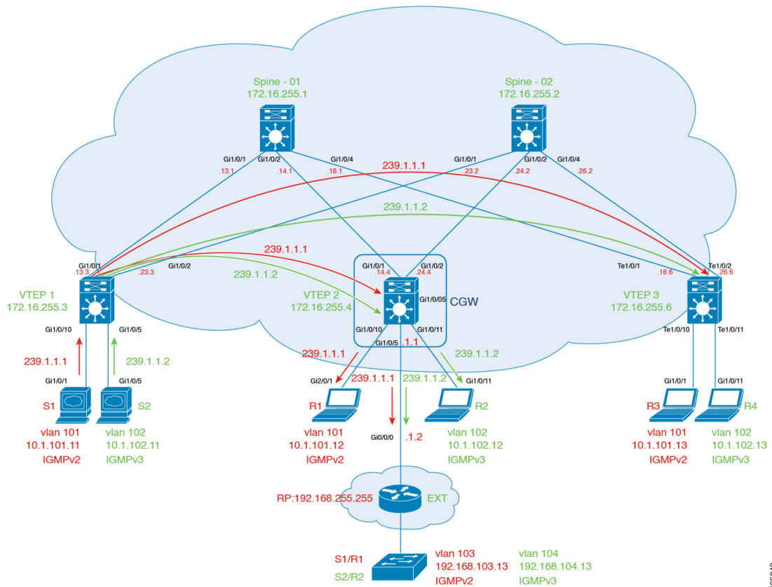
Figure 61: Topology for Optimized Layer 2 Overlay Multicast Interworking with External Network for IPv4 Traffic
