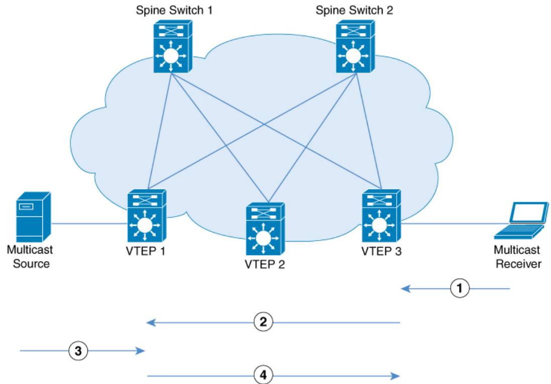
Figure 28: PIM Source Specific Mode
