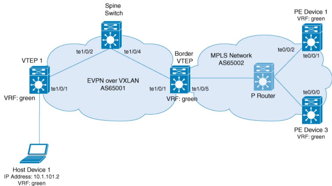
Figure 39: Layer 3 External Connectivity with MPLS Layer 3 VPN through eBGP
