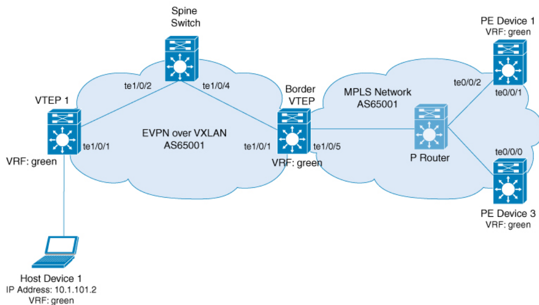
Figure 38: Layer 3 External Connectivity with MPLS Layer 3 VPN through iBGP
