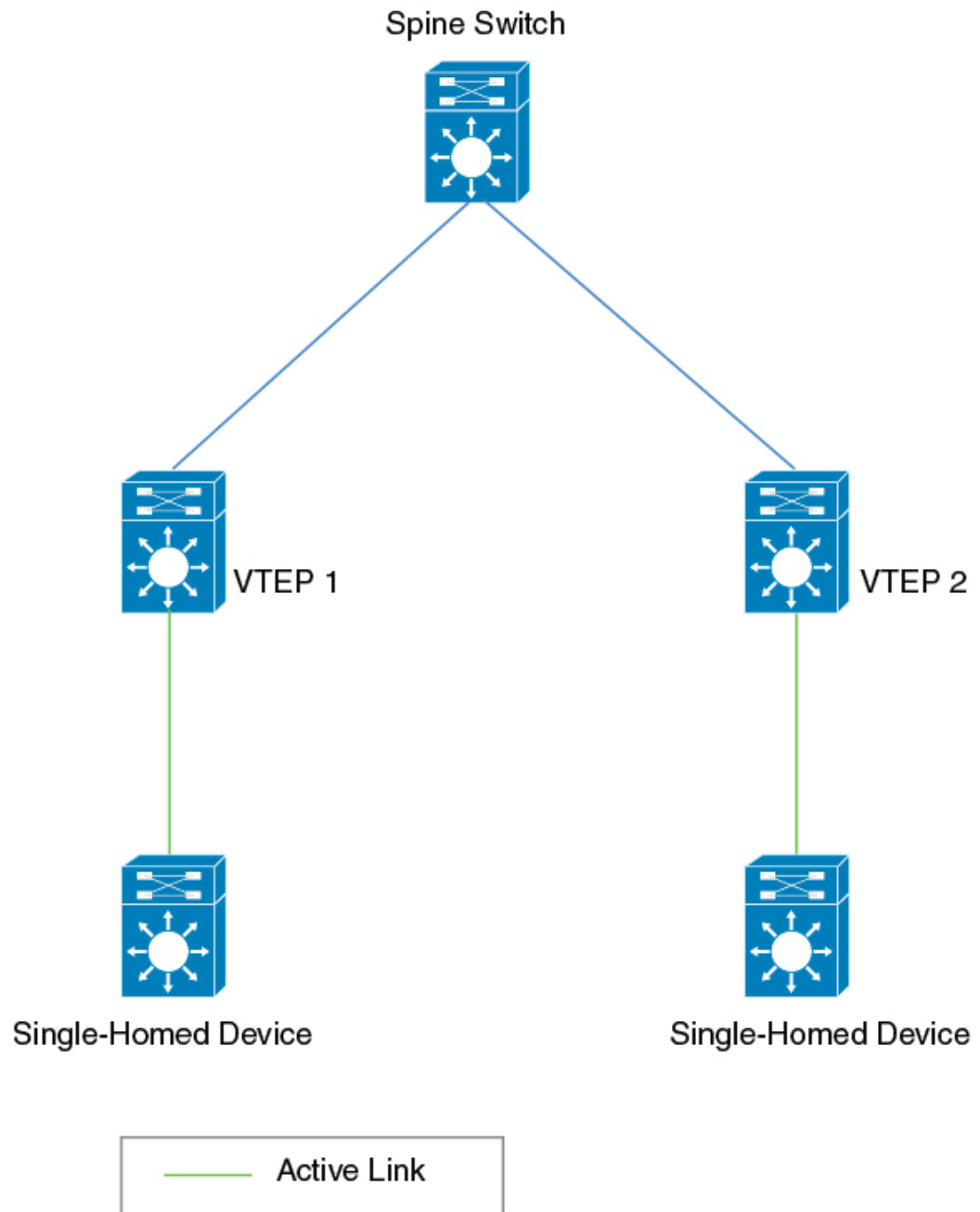
Figure 40: Single-Homed Topology
