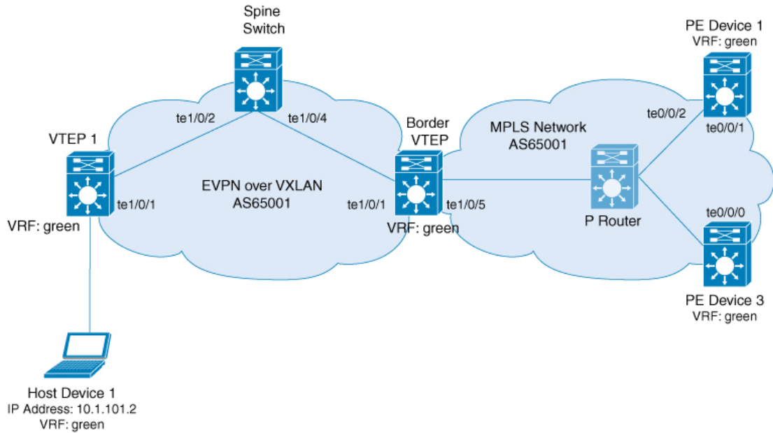
Figure 35: Layer 3 External Connectivity with MPLS Layer 3 VPN
