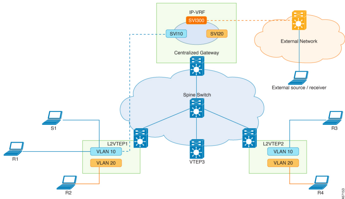
Figure 56: Topology to show Layer 2 Overlay Multicast Traffic Handoff to an External Network
