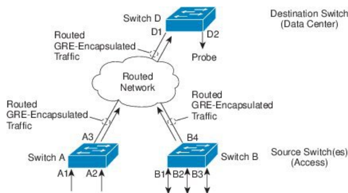
Figure 9: ERSPAN Configuration
