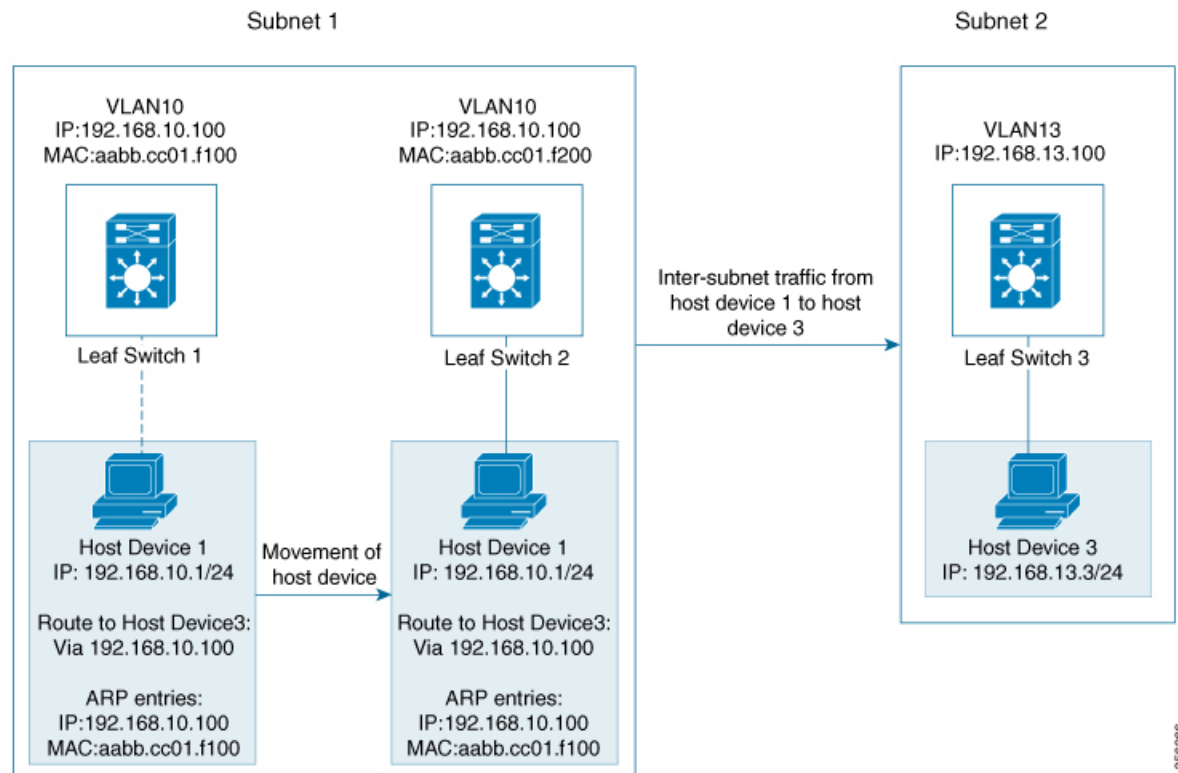
Figure 9: Distributed Gateway Topology
