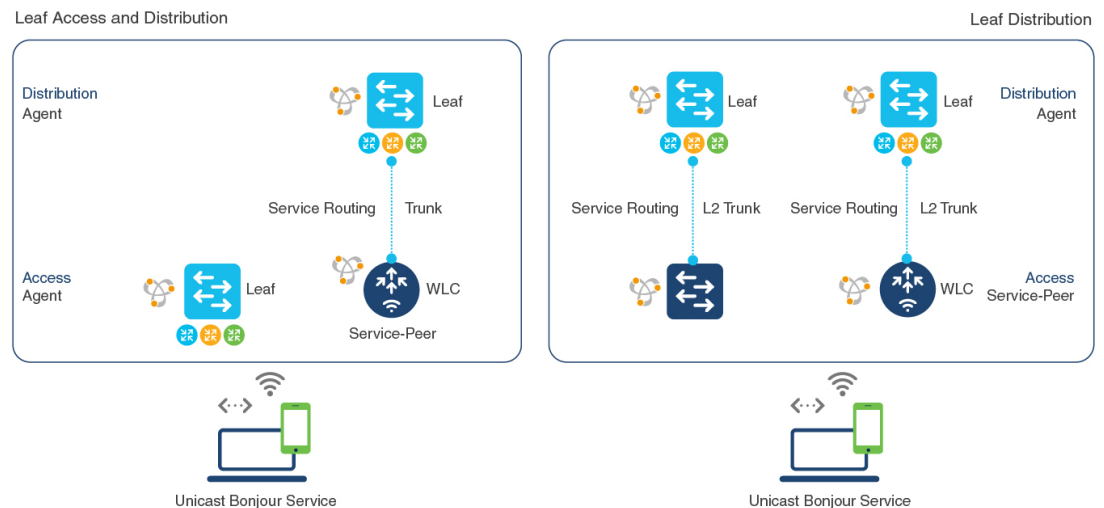
Figure 66: Local Area Bonjour Unicast Mode for Wired and Wireless Local Mode Networks
