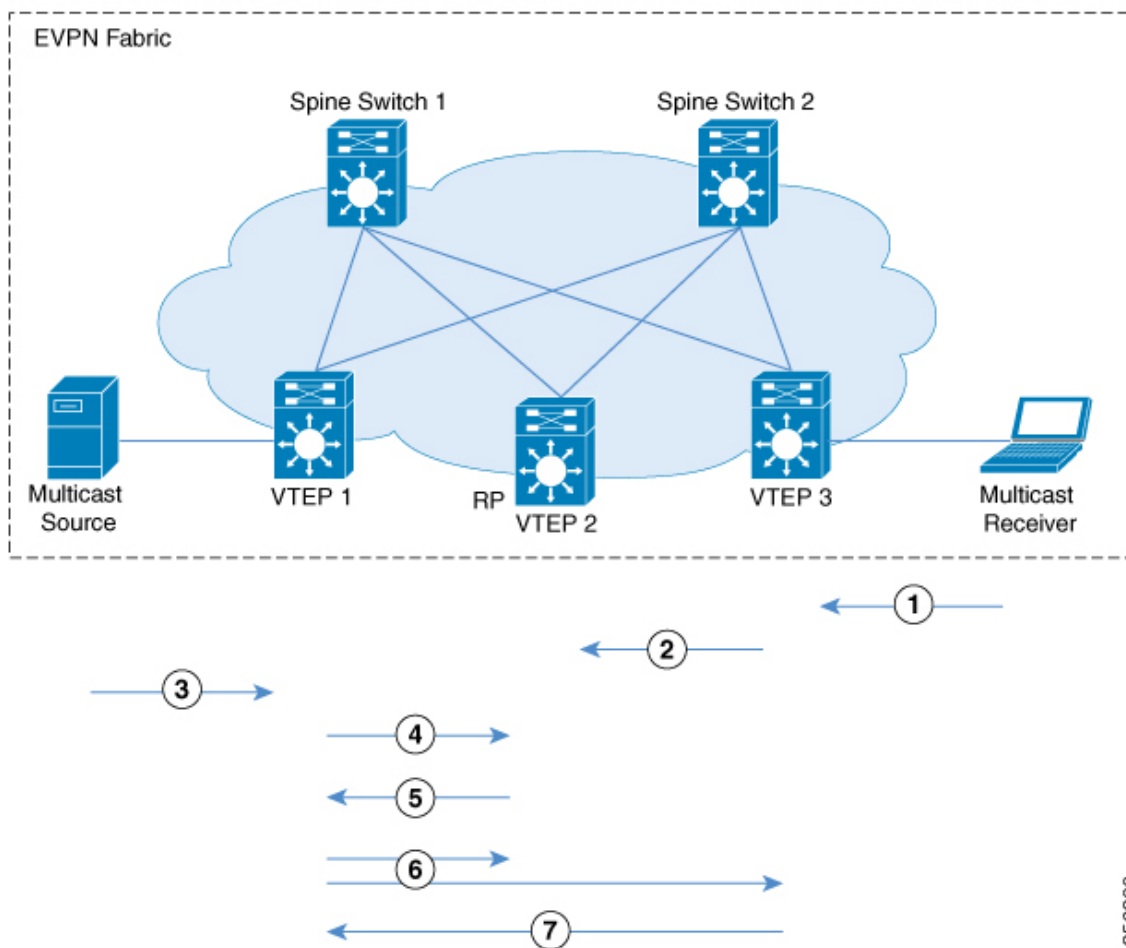
Figure 20: PIM Sparse Mode with RP Inside the BGP EVPN VXLAN Fabric
