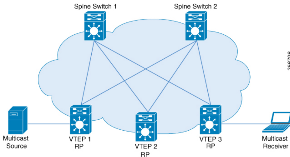
Figure 15: Anycast RP in the Overlay Network
