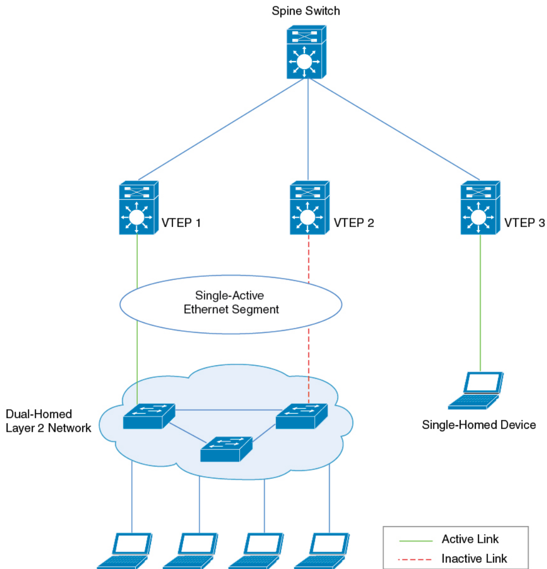
Figure 36: Dual-Homed Network Topology
