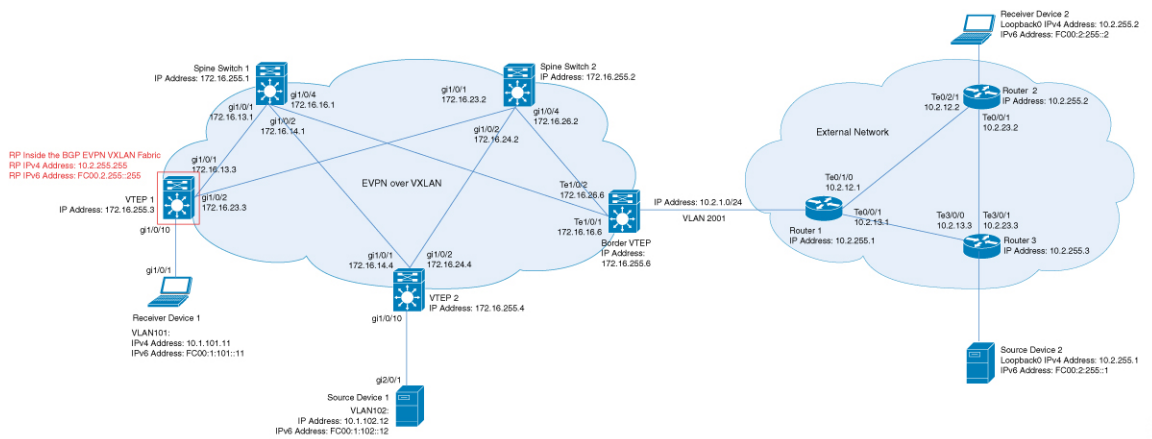
Figure 24: TRM with PIM-SM when the RP is Inside the BGP EVPN VXLAN Fabric
