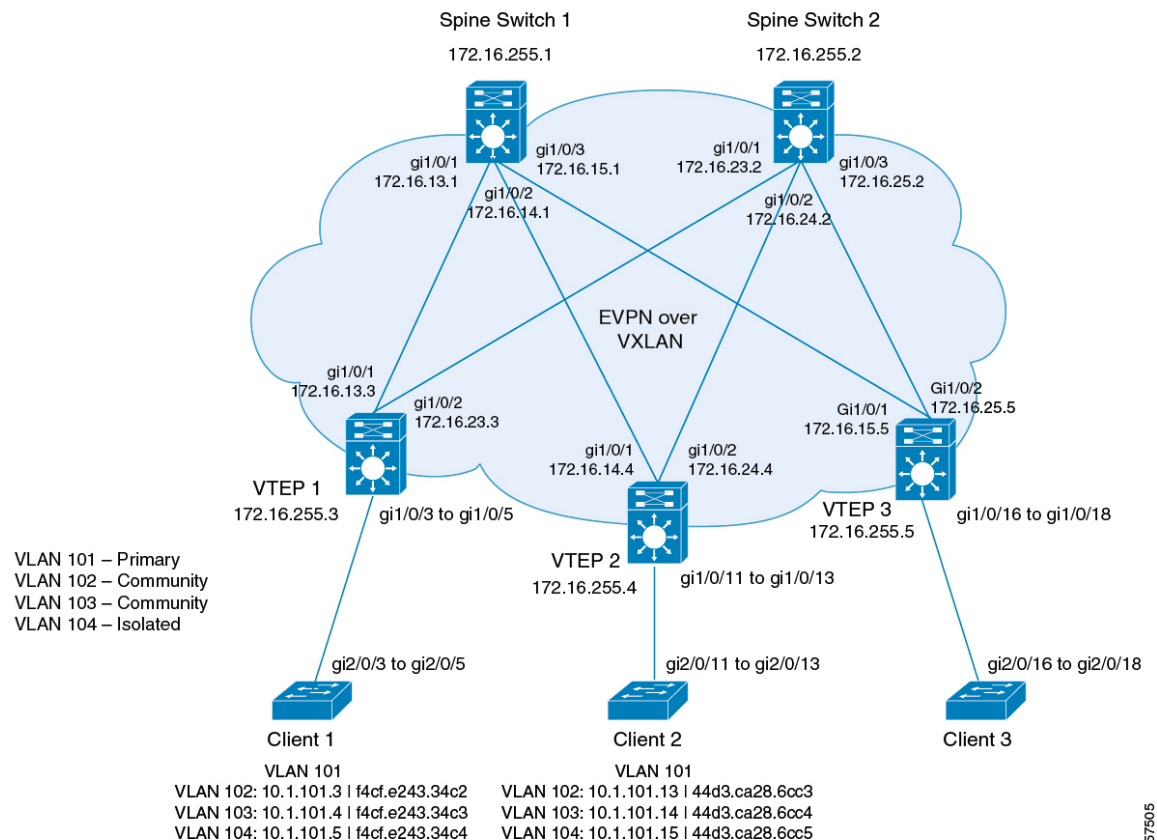
Figure 47: Private VLANs in a BGP EVPN VXLAN Fabric
