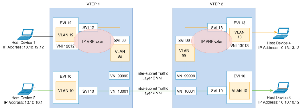
Figure 51: Movement of traffic in an EVPN VXLAN network through Layer2 and Layer 3 VNIs
