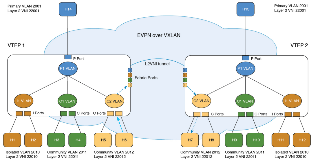
Figure 43: Unicast Traffic from Community Port: H6 to H7
