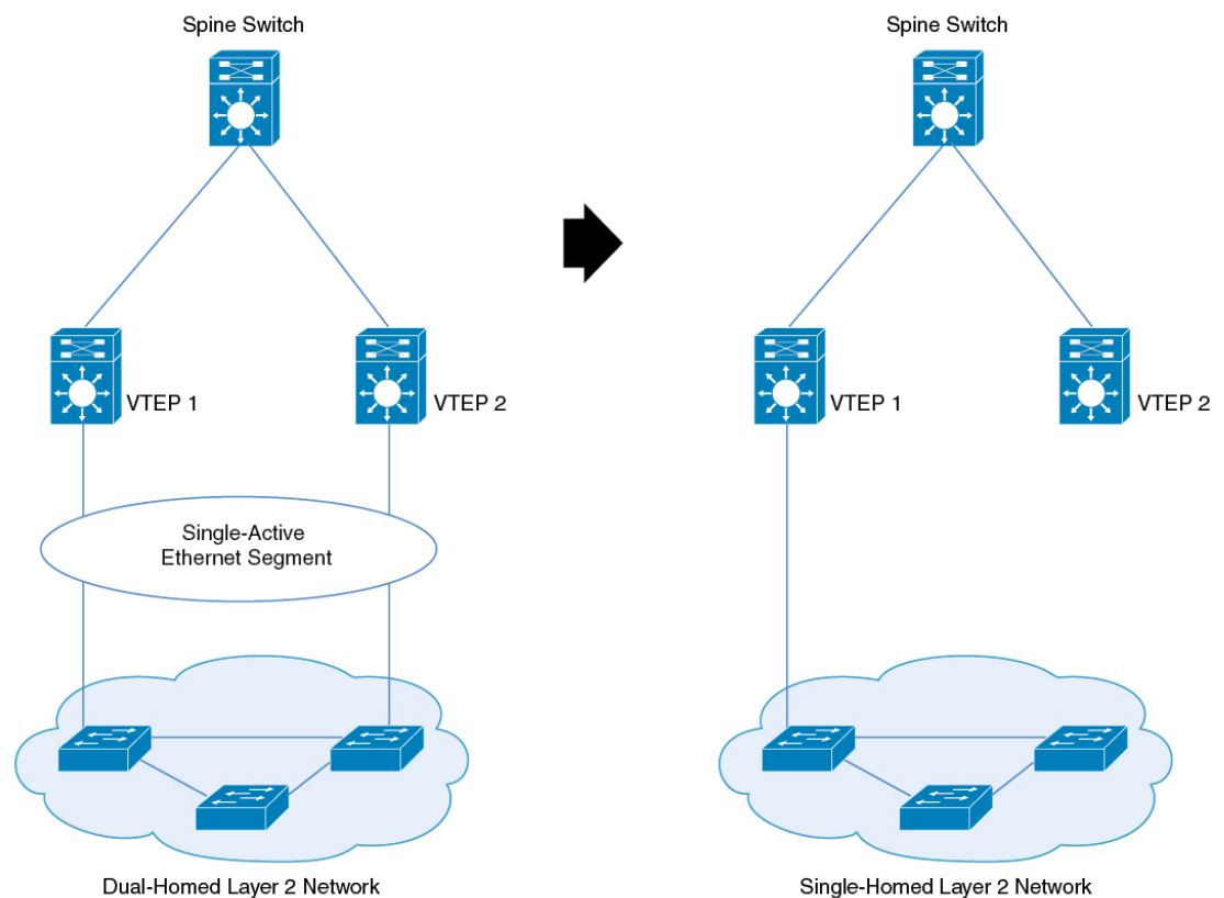
Figure 38: Migration from a Single-Active Dual-Homed Network to a Single-Homed Network
