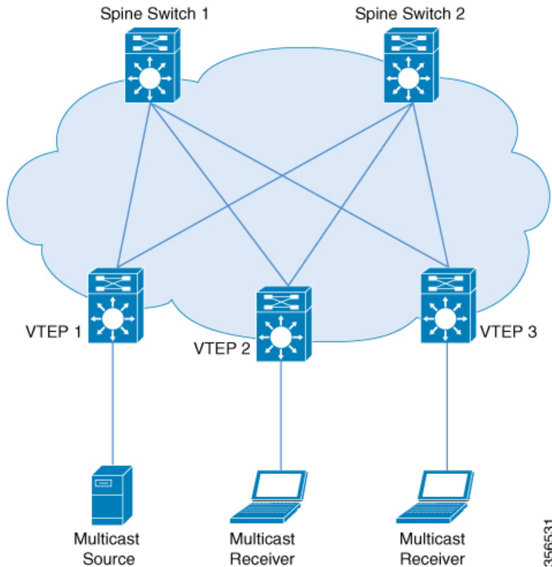
Figure 14: Tenant Routed Multicast Topology
