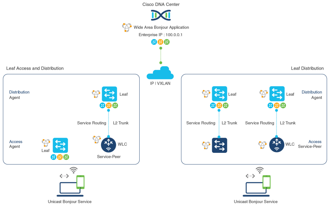
Figure 66: Deployment Model for Wide Area Bonjour over BGP EVPN VXLAN
