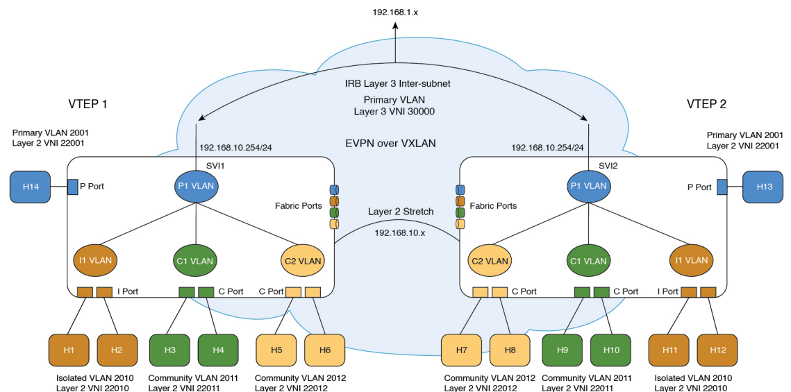
Figure 40: PVLAN Extension in a BGP EVPN VXLAN Fabric
