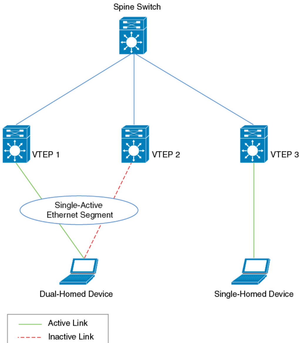
Figure 35: Dual-Homed Device Topology
