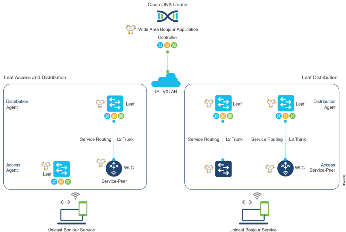
Figure 61: Wide Area Bonjour for Wired and Wireless BGP EVPN Layer 3 Overlay Networks
