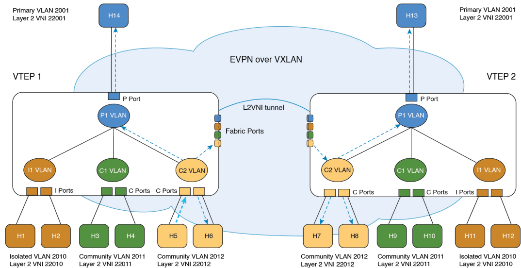
Figure 46: BUM Traffic from Community Port (H5)
