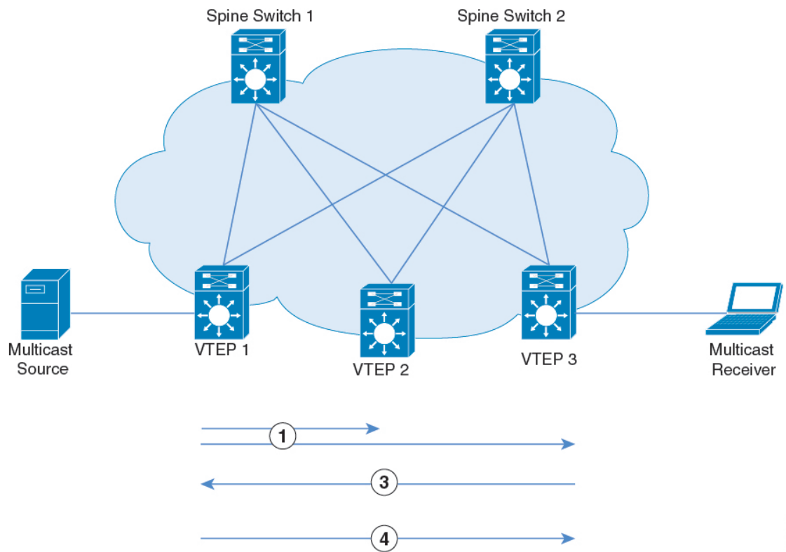
Figure 23: Data MDT Mode
