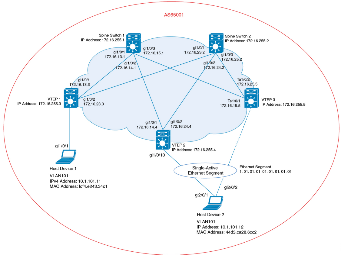
Figure 39: Dual-Homing with Single-Active Redundancy in a BGP EVPN VXLAN Fabric
