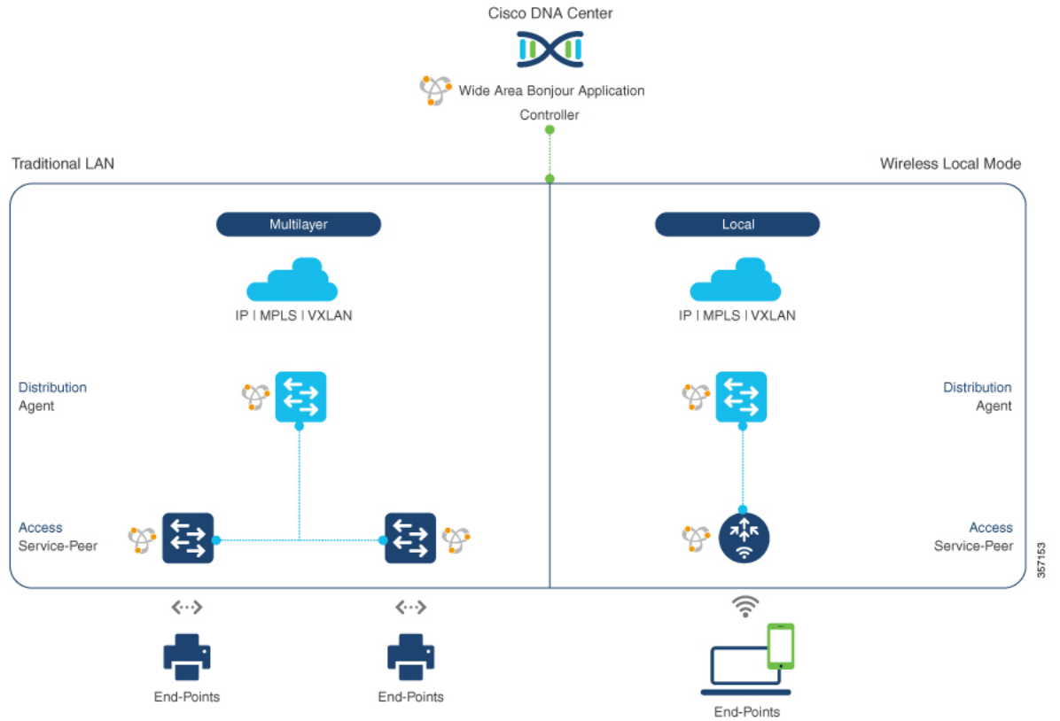
Figure 53: Enterprise Traditional LAN Network Design
