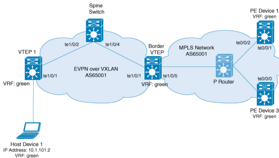
Figure 32: Layer 3 External Connectivity with MPLS Layer 3 VPN through iBGP
