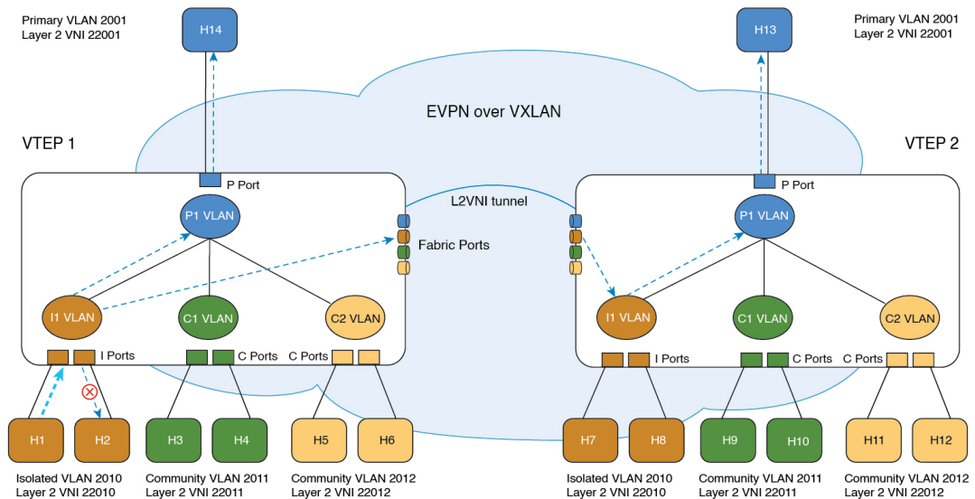
Figure 45: BUM Traffic from Isolated Port (H1)
