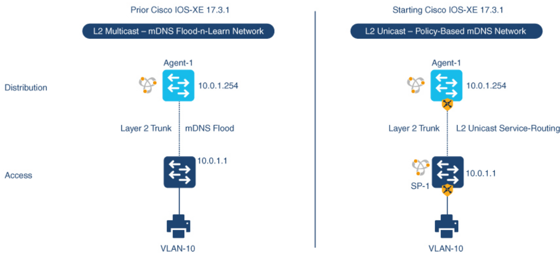
Figure 15: Migration from mDNS Flood to Layer 2 Service-Routing Unicast Mode
