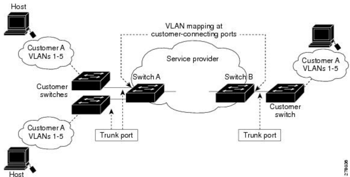
Figure 32: Mapping Customer VLANs to Service-Provider VLANs
