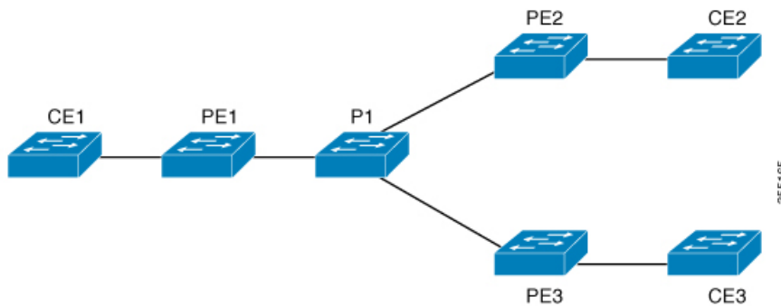
Figure 3: VPLS Topology
