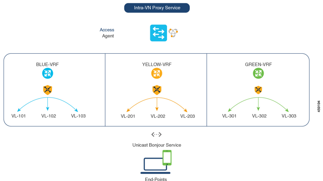
Figure 5: Intra-VN Service Proxy
