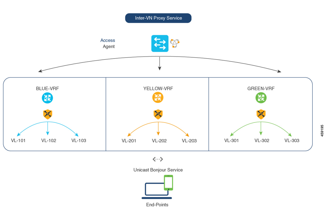
Figure 6: Inter-VN Proxy Service
