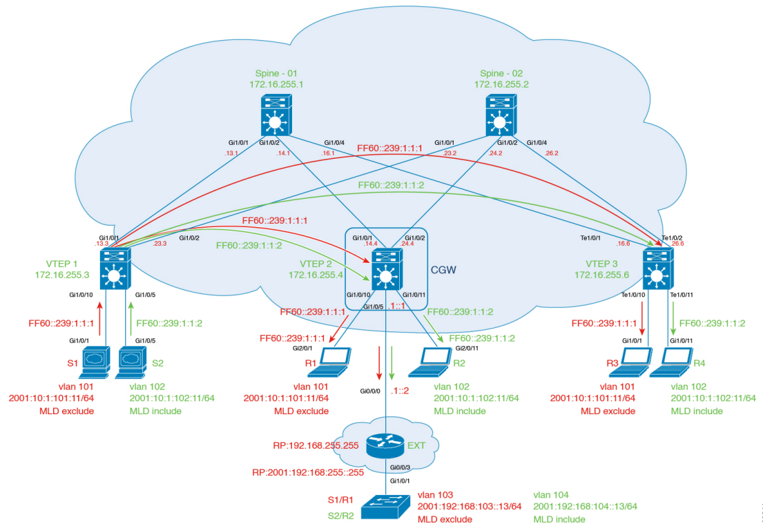
Figure 33: Topology for Optimized Layer 2 Overlay Multicast Interworking with External Network for IPv6 Traffic
