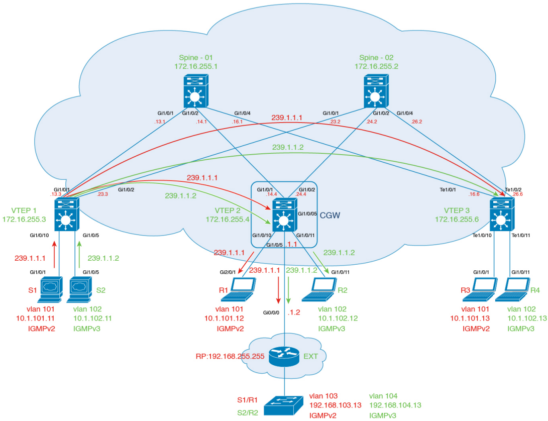
Figure 32: Topology Showing Optimized Layer 2 Overlay Multicast Interworking with External Network for IPv4 Traffic
