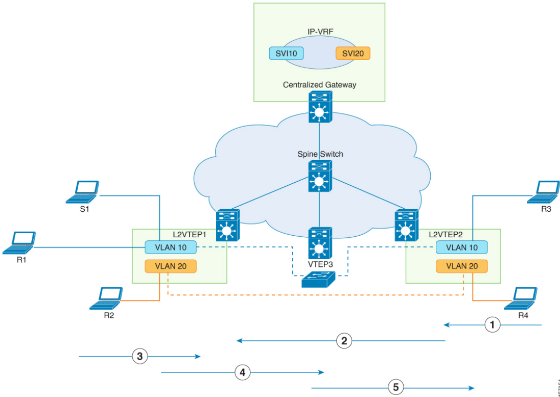
Figure 25: Topology Showing Layer 2 Overlay Multicast Traffic Within a VLAN
