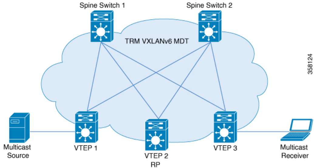
Figure 77: VTEP as an RP for IPv4 and IPv6 Overlay
