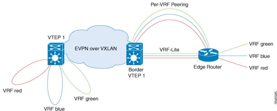
Figure 49: Layer 3 External Connectivity with VRF-Lite
