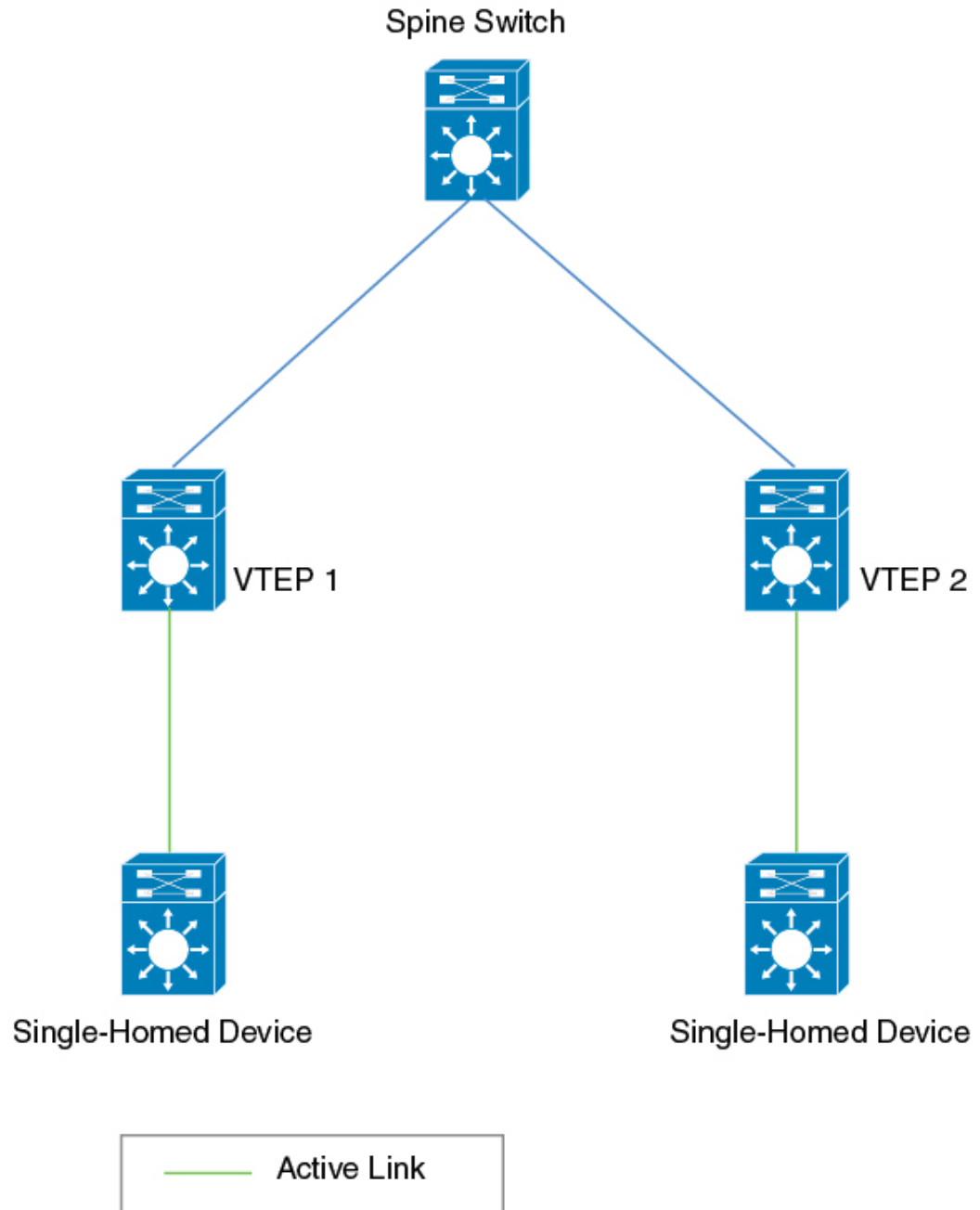
Figure 55: Single-Homed Topology
