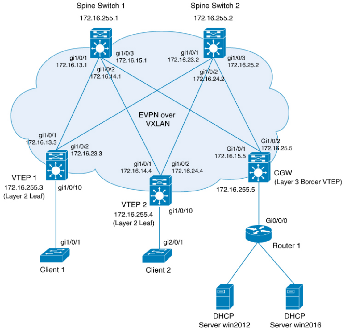
Figure 19: Layer 3 Gateway Configured on Border VTEP
