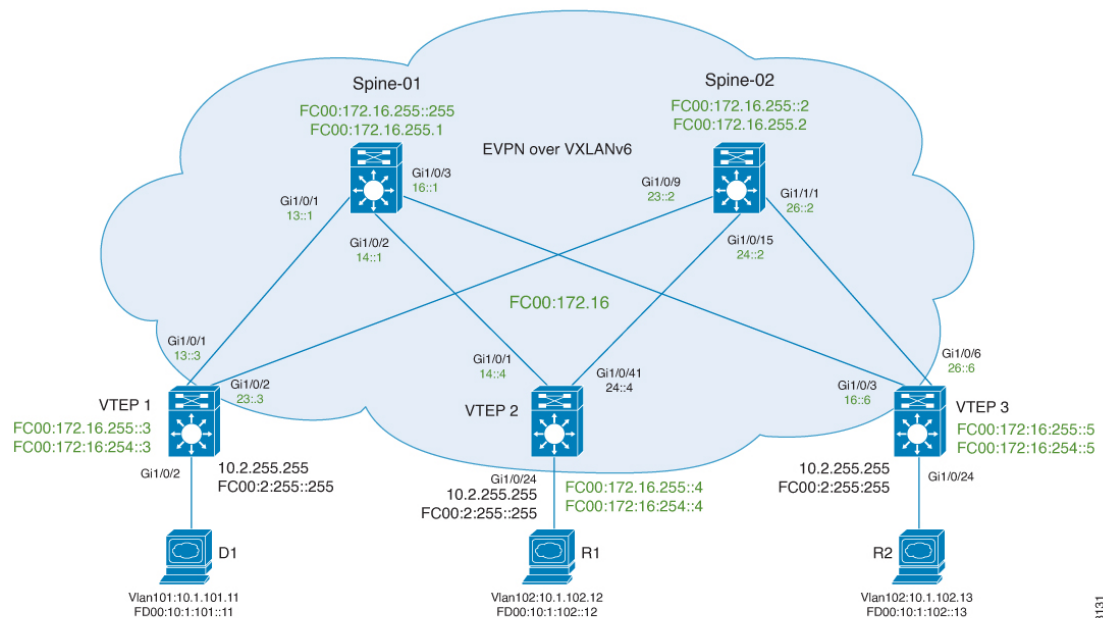
Figure 84: TRM with PIM-SM with Anycast RP over VXLANv6 Fabric
