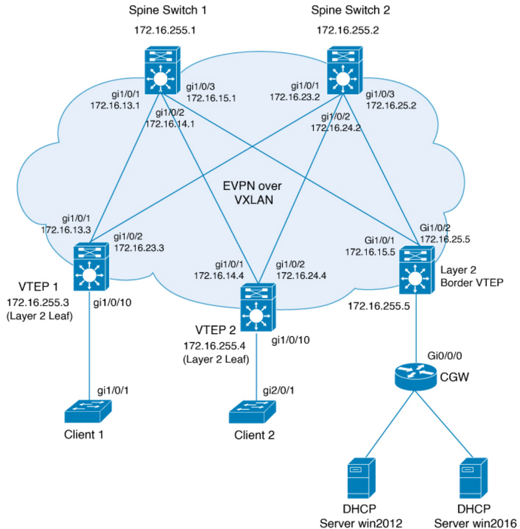
Figure 20: Layer 3 Gateway Configured on External Router
