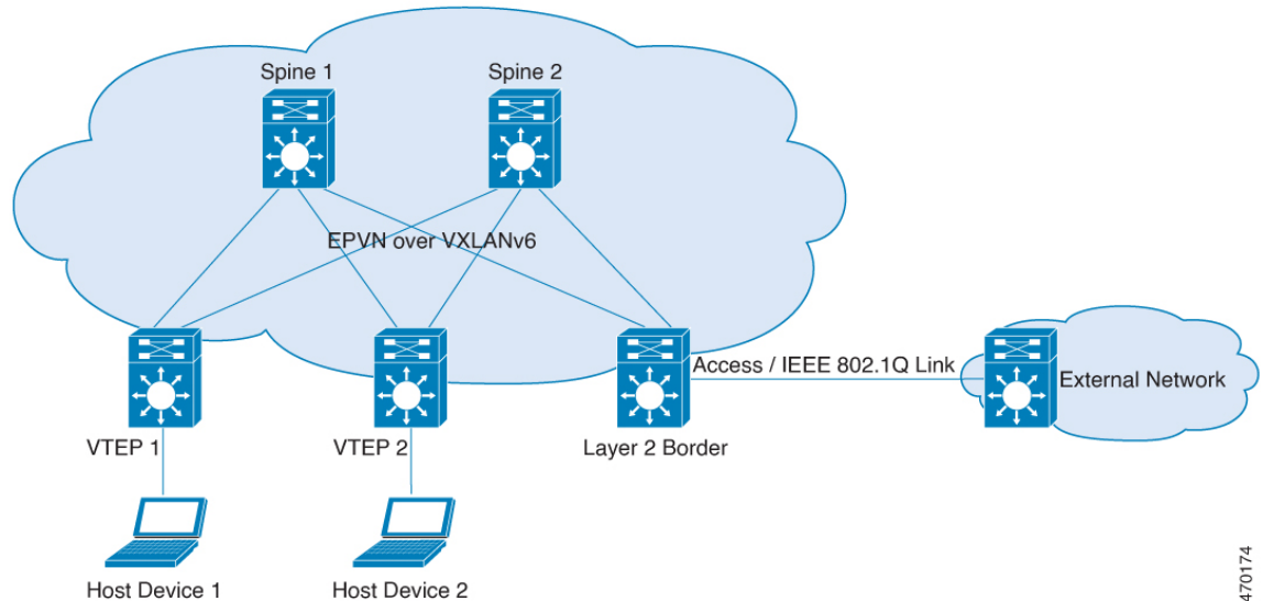
Figure 64: EVPN VXLANv6 Fabric with Layer 2 Gateway
