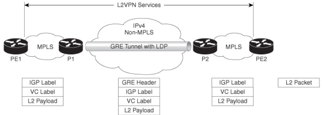
Figure 3: P-to-P Tunneling
