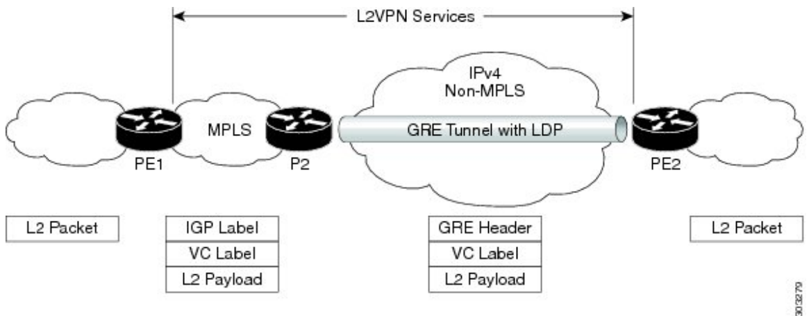
Figure 2: P-to-PE Tunneling
