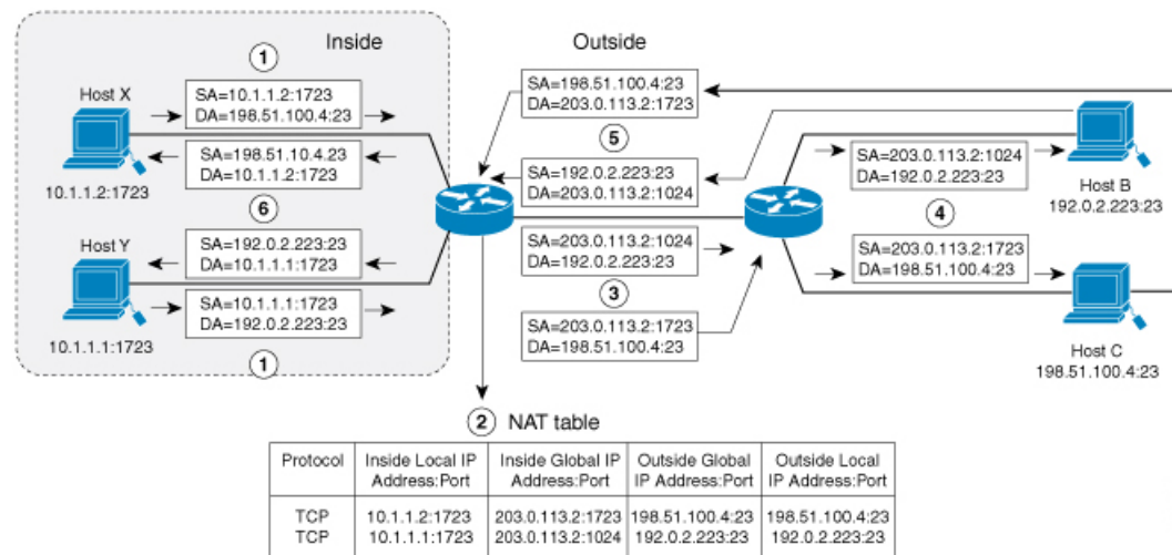
Figure 4: PAT / NAT Overloading Inside Global Addresses
