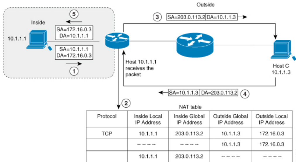
Figure 5: NAT Translating Overlapping Addresses
