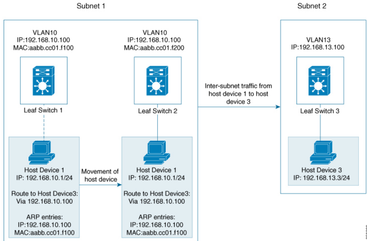
Figure 10: Distributed Gateway Topology
