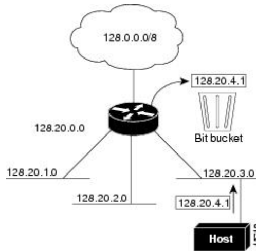
Figure 3: No IP Classless Routing
