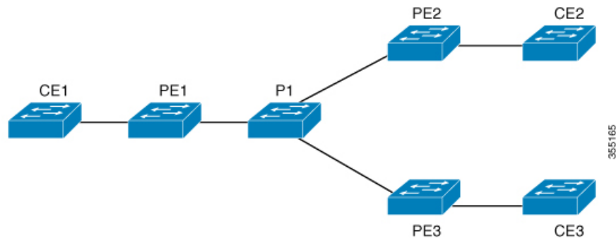
Figure 4: VPLS Topology
