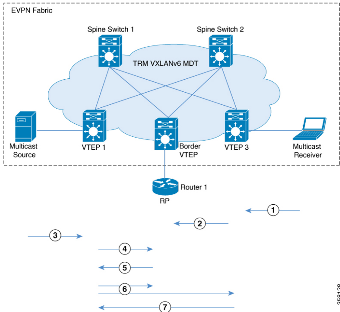
Figure 80: PIM Sparse Mode with RP Outside the BGP EVPN VXLAN Fabric
