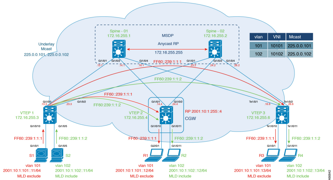
Figure 29: Topology for Optimized Layer 2 Overlay Multicast for IPv6 with Underlay Multicast Replication
