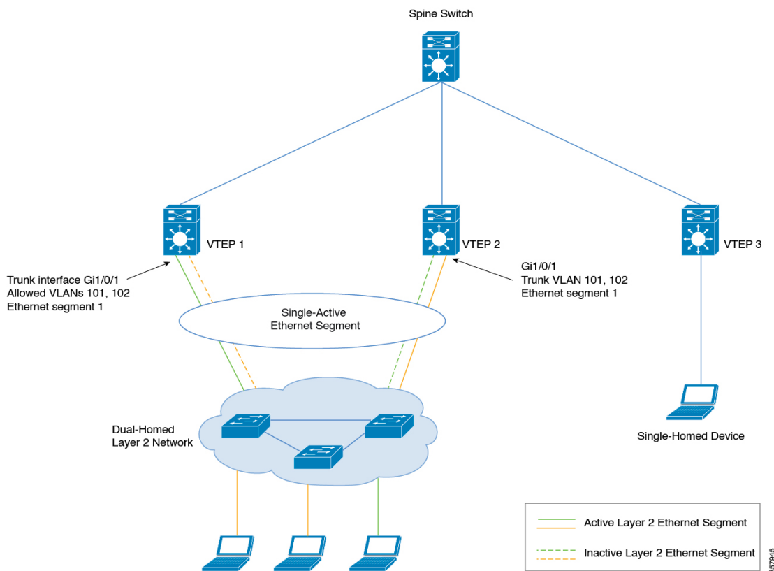
Figure 55: Dual-Homed Network Topology
