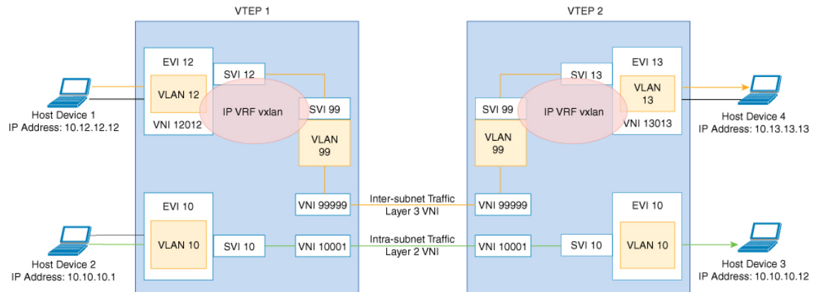
Figure 87: Movement of traffic in an EVPN VXLAN network through Layer2 and Layer 3 VNIs
