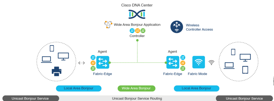
Figure 92: Cisco SD-Access Wired and Wireless Network Design
