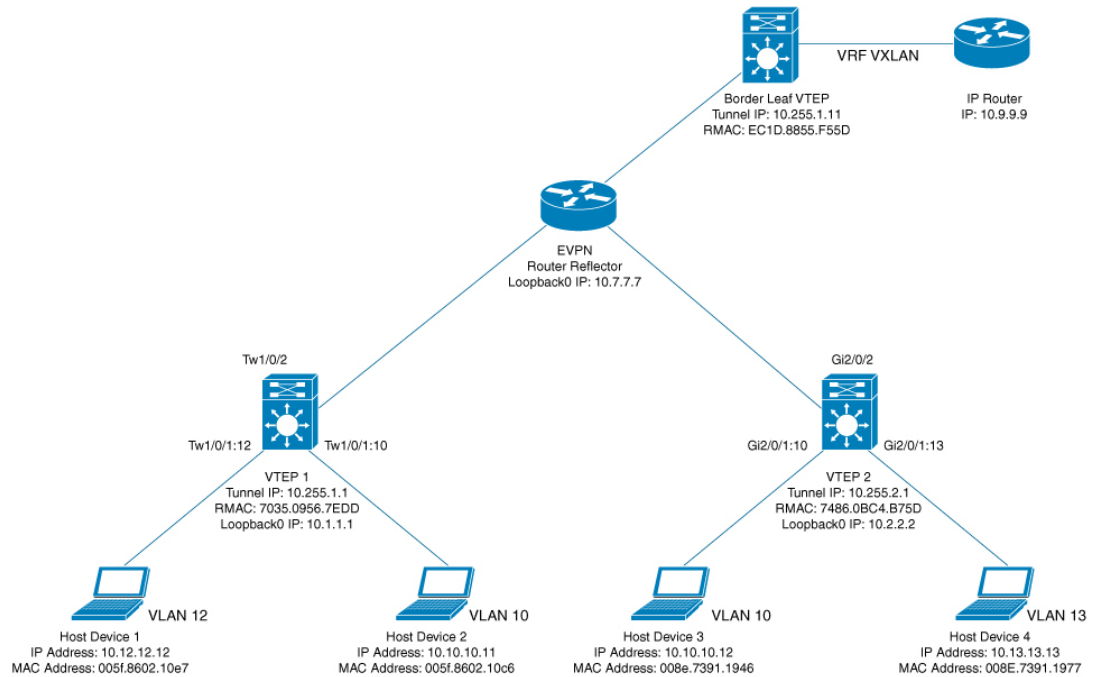
Figure 85: EVPN VXLAN Topology
