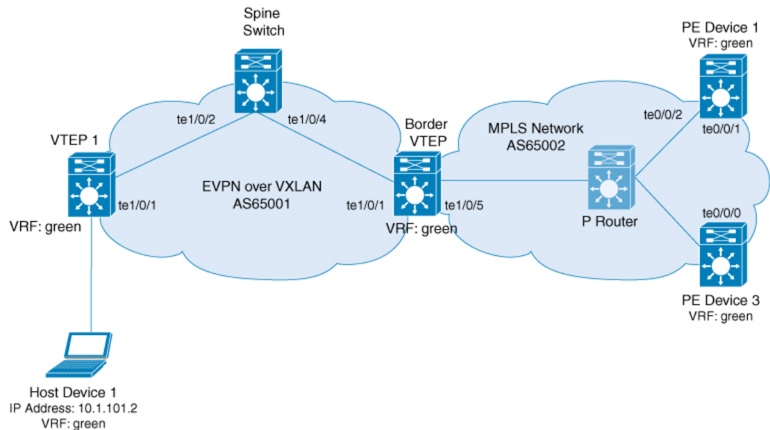
Figure 52: Layer 3 External Connectivity with MPLS Layer 3 VPN through eBGP
