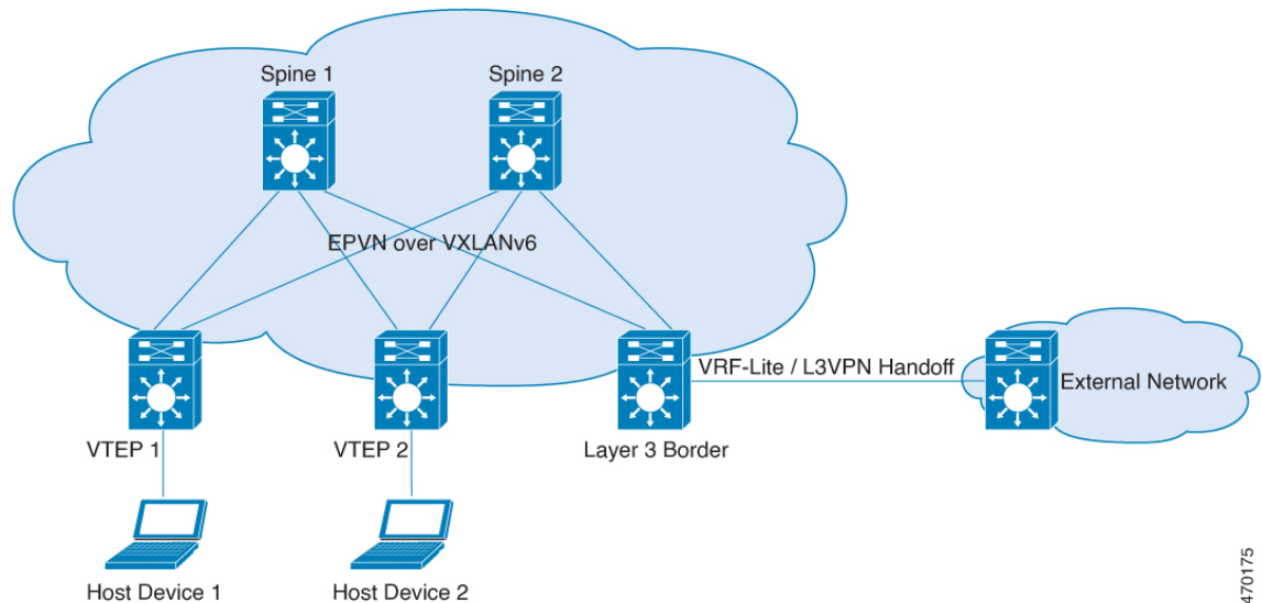
Figure 68: BGP EVPN VXLANv6 Fabric with Distributed Anycast Gateway
