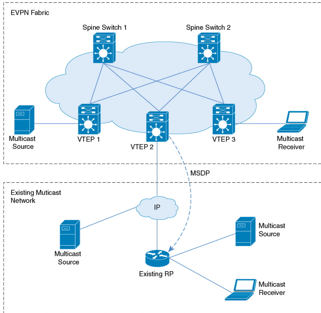
Figure 34: Anycast RP with IPv4 Overlay in an Existing Multicast Network
