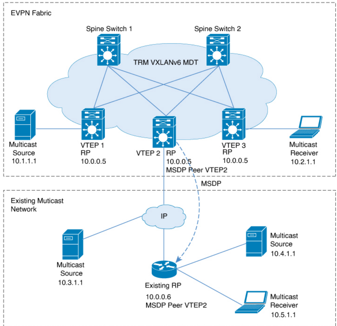
Figure 73: Anycast RP with IPv4 Overlay in an Existing Multicast Network
