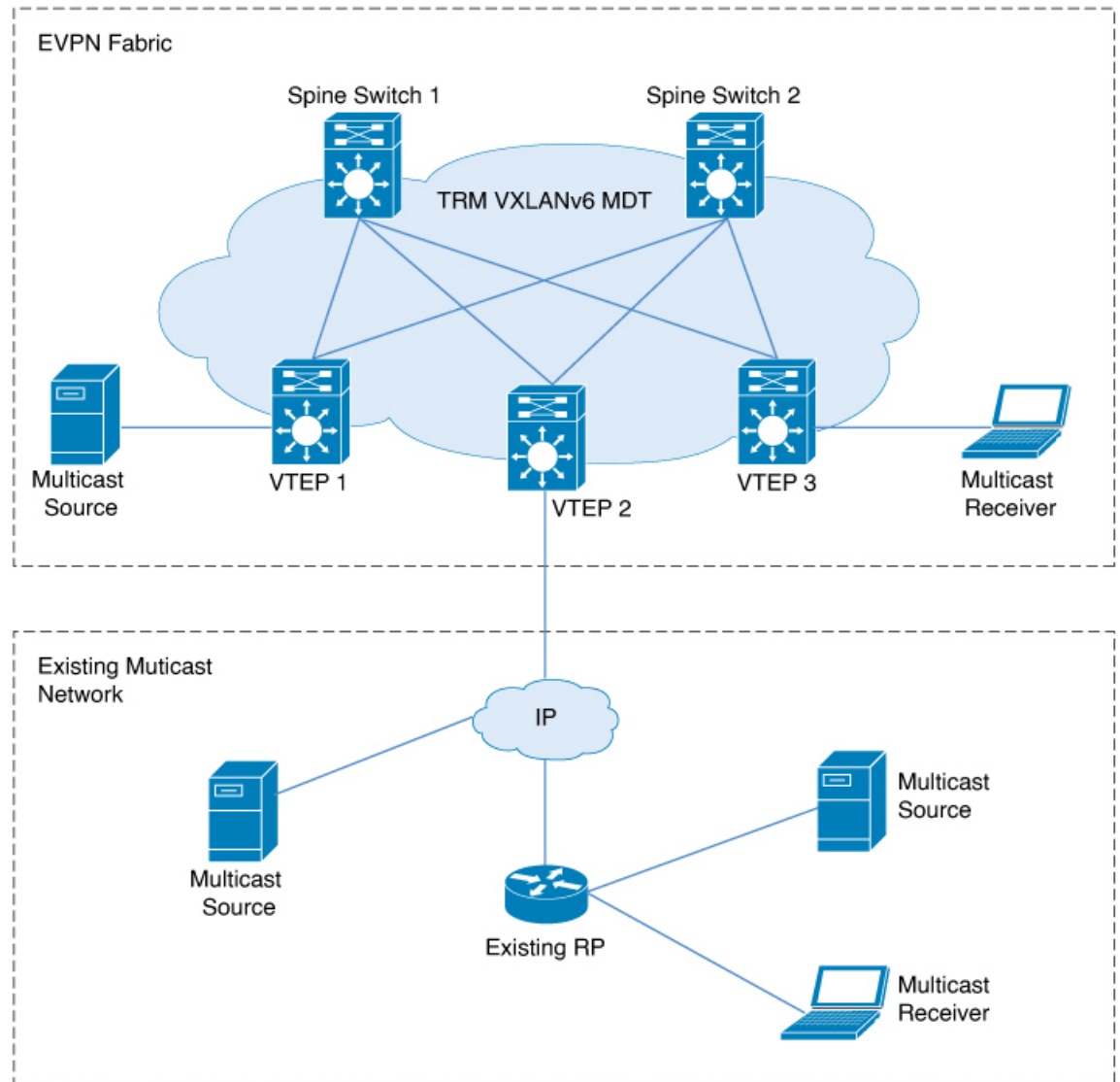
Figure 77: RP Outside the BGP EVPN VXLAN Fabric with an Existing Multicast Network for IPv4 and IPv6 Overlay
