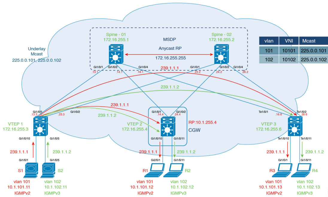
Figure 28: Topology for Optimized Layer 2 Overlay Multicast for IPv4 with Underlay Multicast Replication
