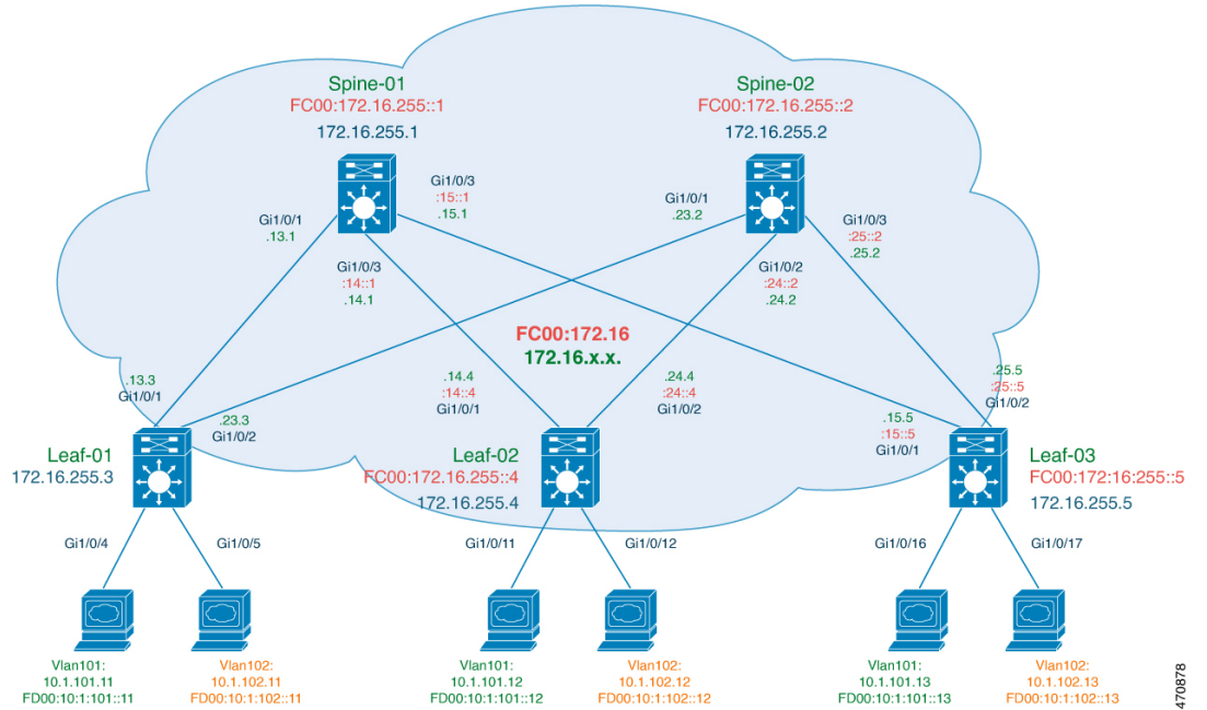
Figure 70: BGP EVPN VXLAN with a Dual Stack Underlay
