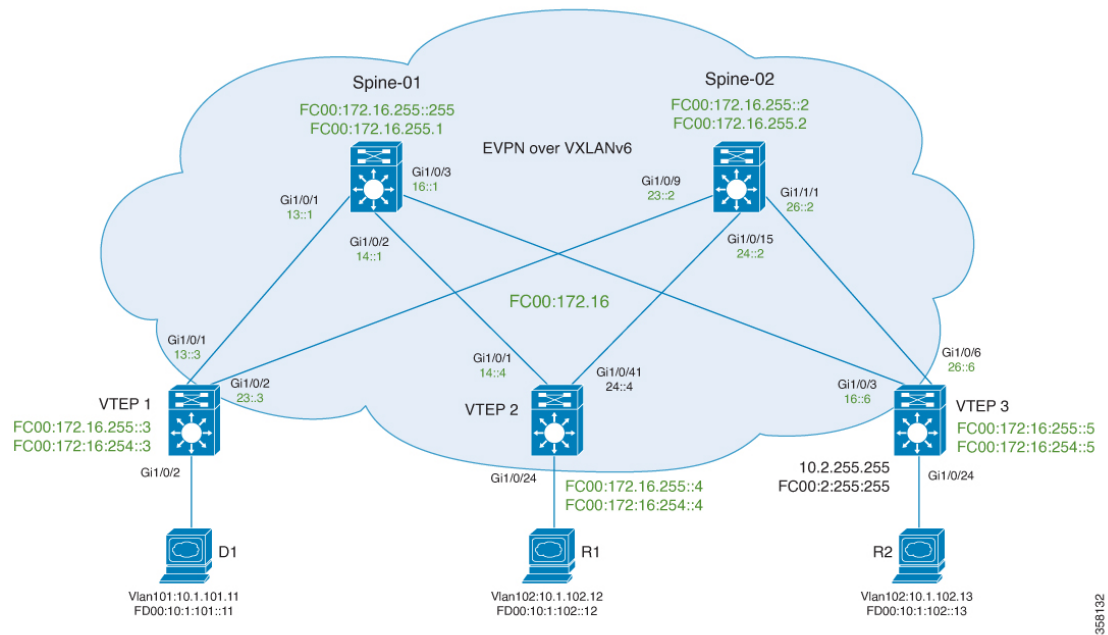
Figure 83: TRM with PIM-SM when the RP is Inside the VXLANv6 Fabric
