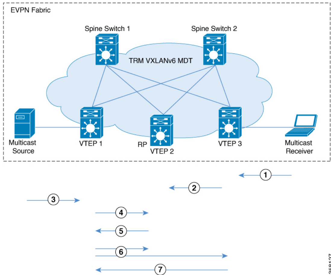
Figure 79: PIM Sparse Mode with RP Inside the BGP EVPN VXLAN Fabric
