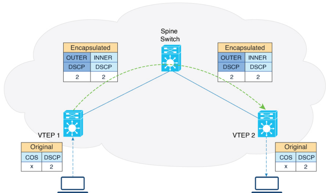
Figure 20: EVPN VXLAN Traffic without a QoS Policy
