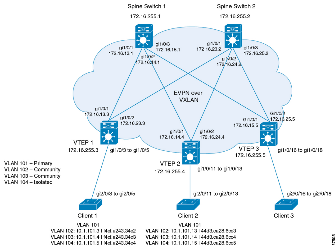
Figure 66: Private VLANs in a BGP EVPN VXLAN Fabric
