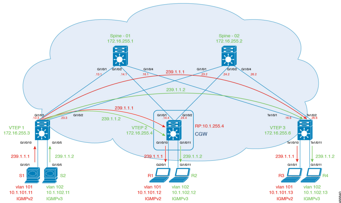
Figure 26: Topology for Optimized Layer 2 Overlay Multicast for IPv4 Traffic with Ingress Replication
