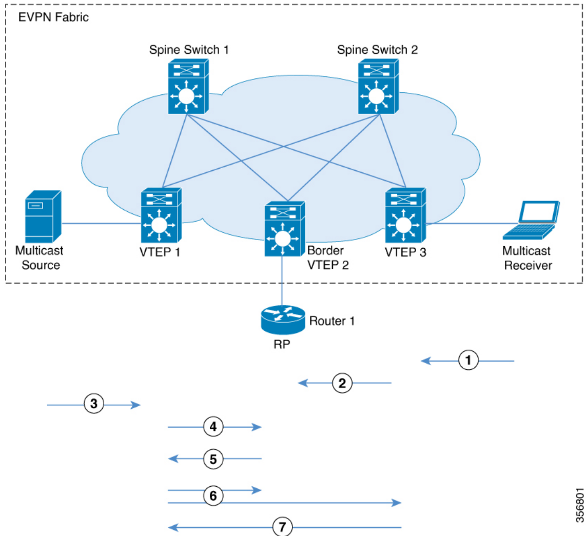
Figure 40: PIM Sparse Mode with RP Outside the BGP EVPN VXLAN Fabric
