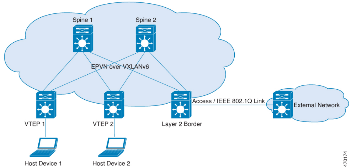
Figure 67: EVPN VXLANv6 Fabric with Layer 2 Gateway
