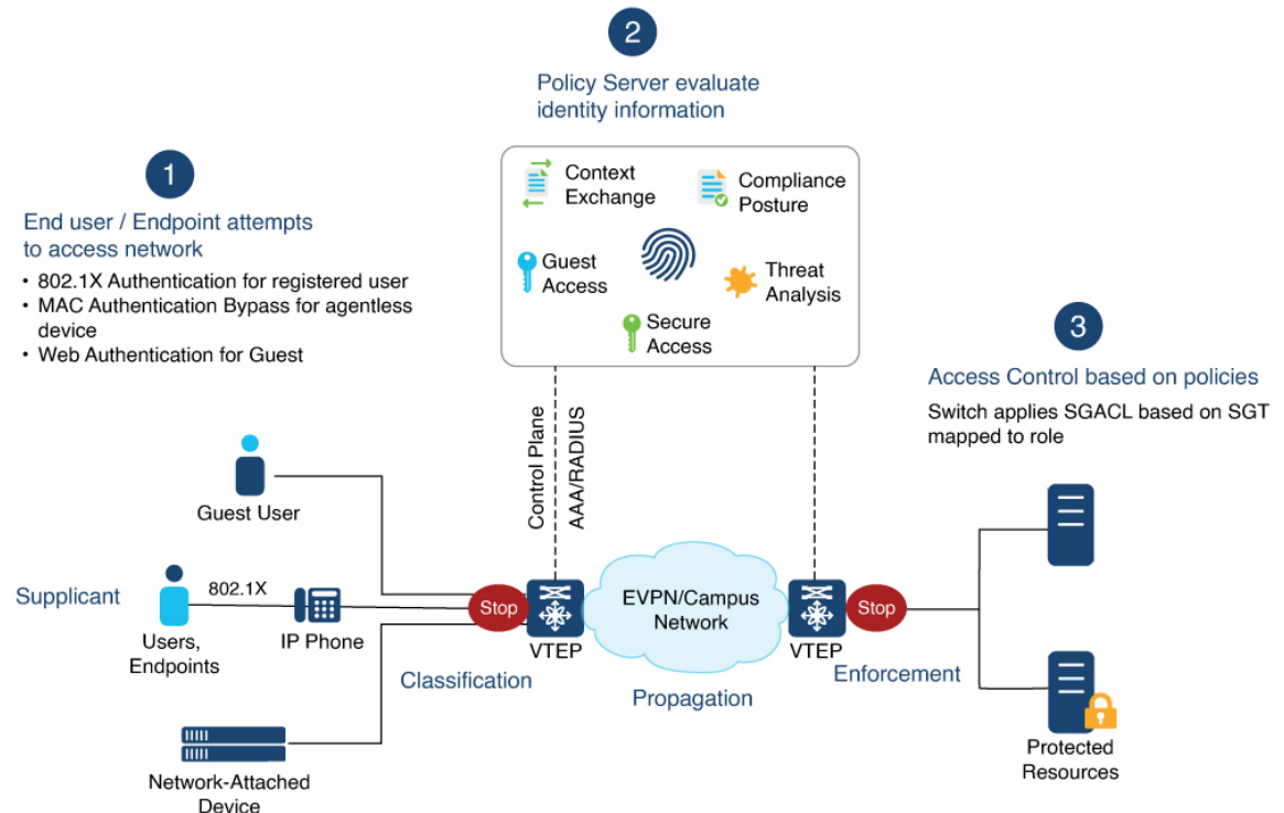
Figure 84: Secure Fabric: BGP EVPN VXLAN Fabric Microsegmentation
