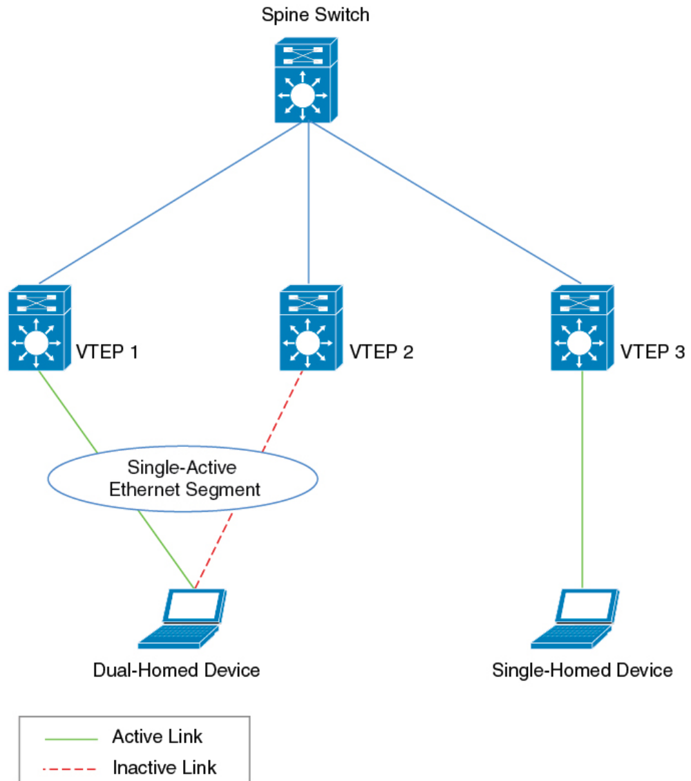
Figure 54: Dual-Homed Device Topology
