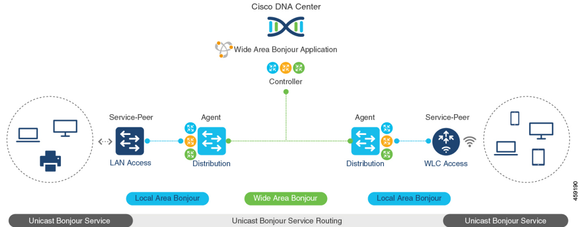
Figure 103: Cisco DNA Service for Bonjour with VRF-Aware Services
