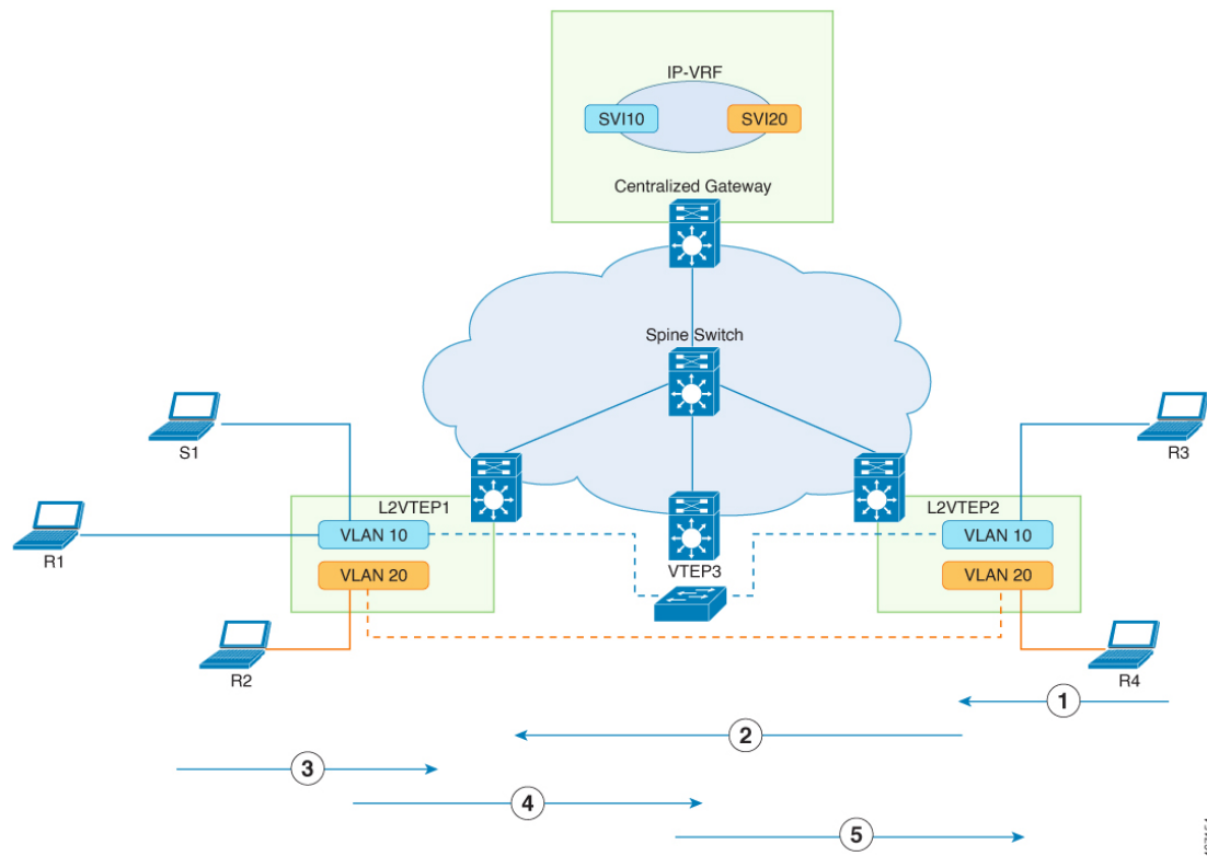
Figure 23: Topology to show Layer 2 Overlay Multicast Traffic within a VLAN
