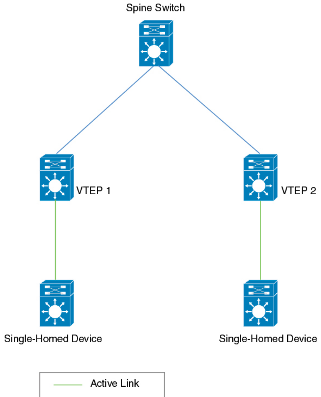
Figure 50: Single-Homed Topology
