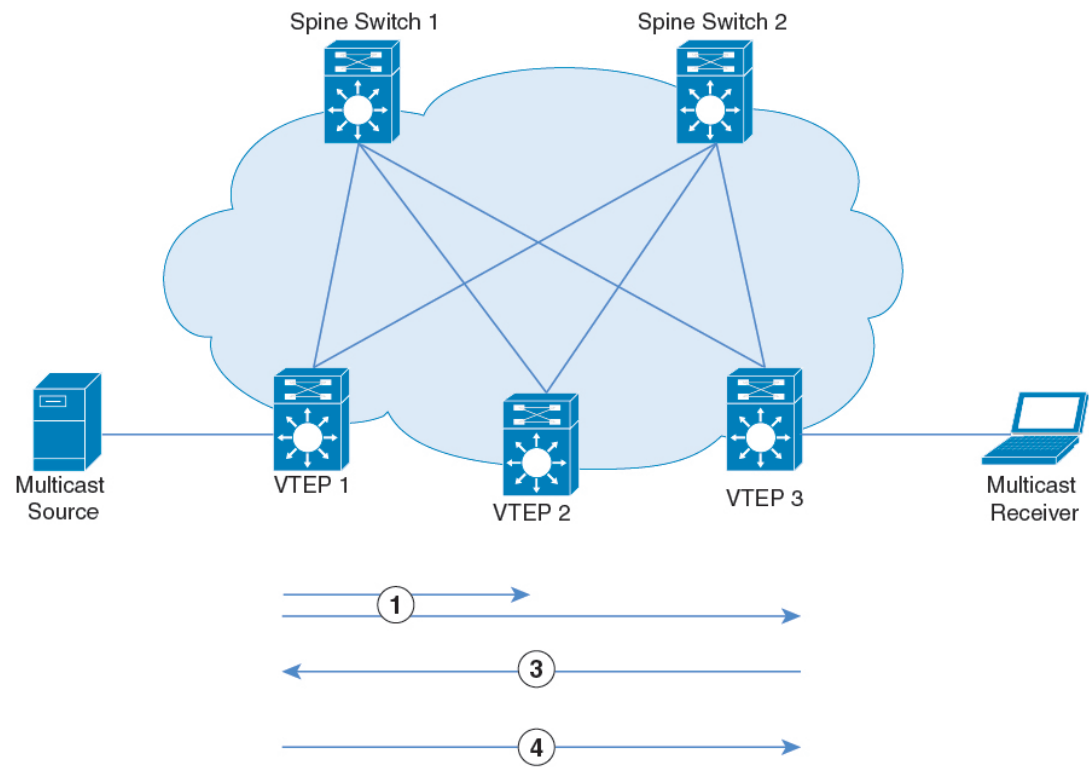
Figure 30: Data MDT Mode
