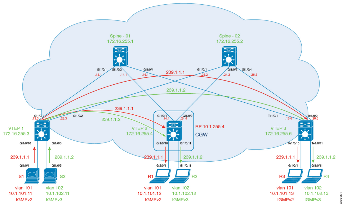
Figure 23: Topology for Optimized Layer 2 Overlay Multicast for IPv4 Traffic with Ingress Replication
