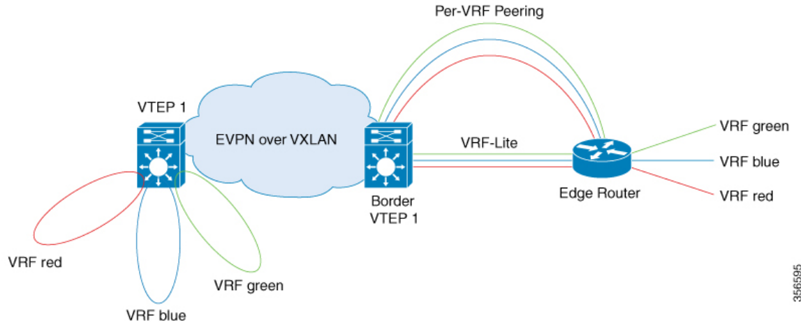
Figure 44: Layer 3 External Connectivity with VRF-Lite
