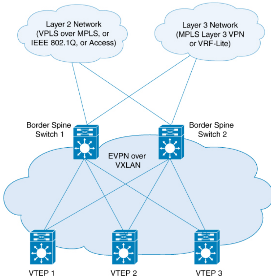
Figure 43: EVPN VXLAN External Connectivity Through a Border Spine Switch
