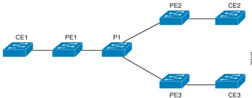
Figure 29: VPLS Topology
