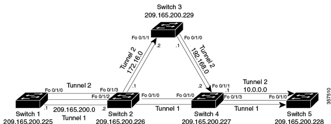
Figure 23: Sample MPLS Traffic Engineering Tunnel Configuration
