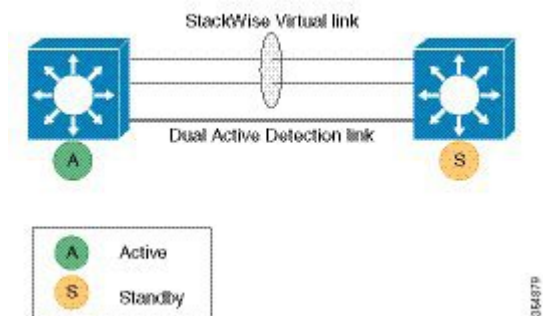
Figure 4: Two-Node Solution
