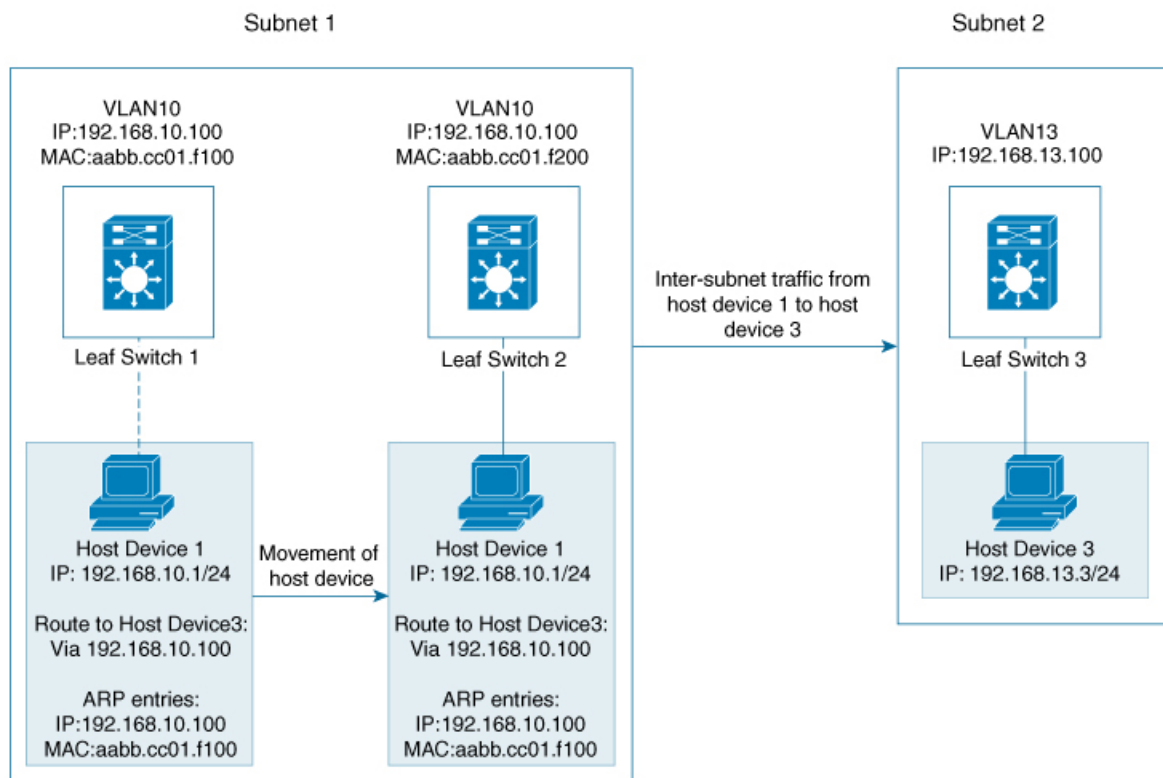
Figure 11: Distributed Gateway Topology
