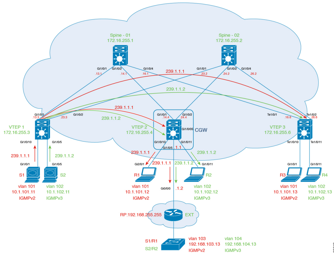
Figure 62: Topology for Optimized Layer 2 Overlay Multicast Interworking with External Network for IPv4 Traffic
