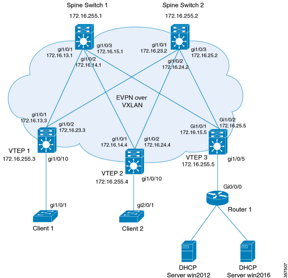
Figure 18: DHCP Relay Deployment in a BGP EVPN VXLAN Fabric
