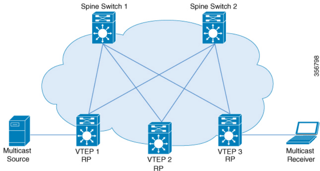
Figure 21: Anycast RP in the Overlay Network
