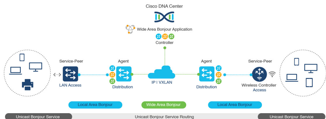
Figure 77: Overlay Bonjour Service for a BGP EVPN-Enabled Enterprise Network
