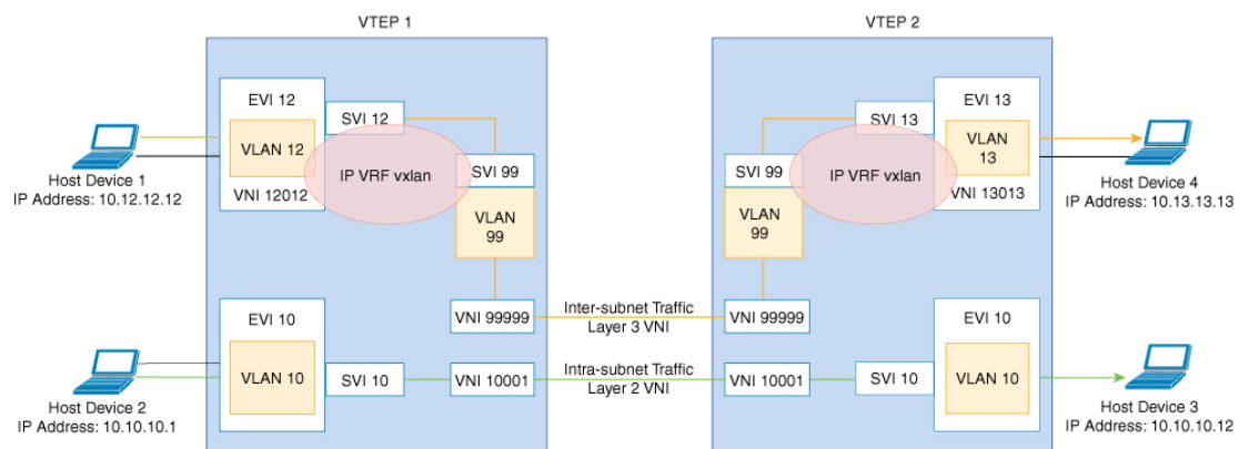
Figure 69: Movement of traffic in an EVPN VXLAN network Through Layer 2 and Layer 3 VNIs
