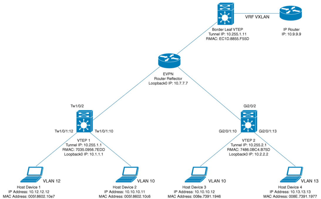
Figure 68: EVPN VXLAN Topology
