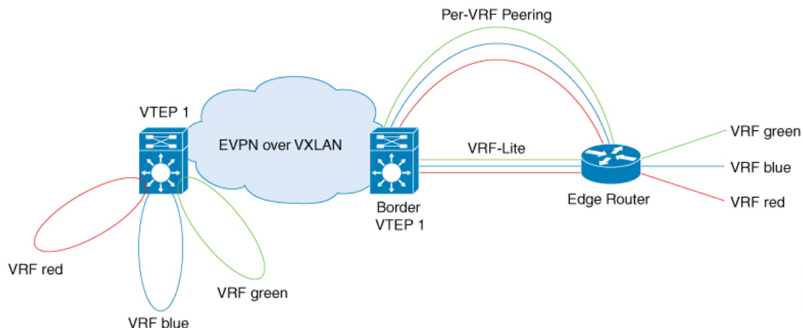
Figure 35: Layer 3 External Connectivity with VRF-Lite
