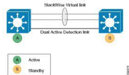
Figure 4: Two-Node Solution
