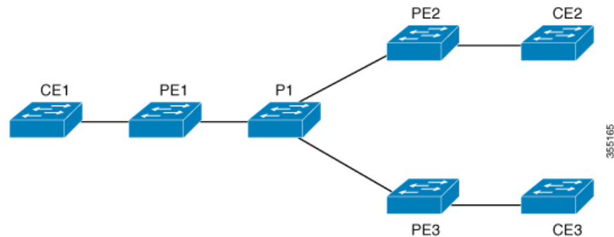
Figure 4: VPLS Topology
