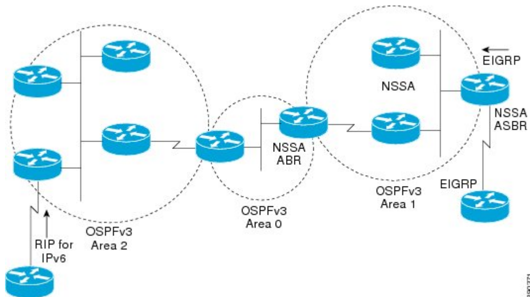
Figure 1: OSPFv3 NSSA
