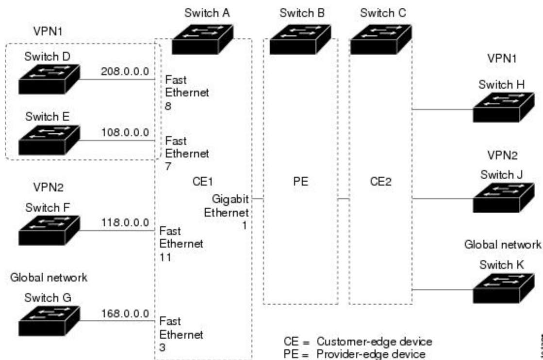
Figure 2: Multi-VRF CE Configuration Example
