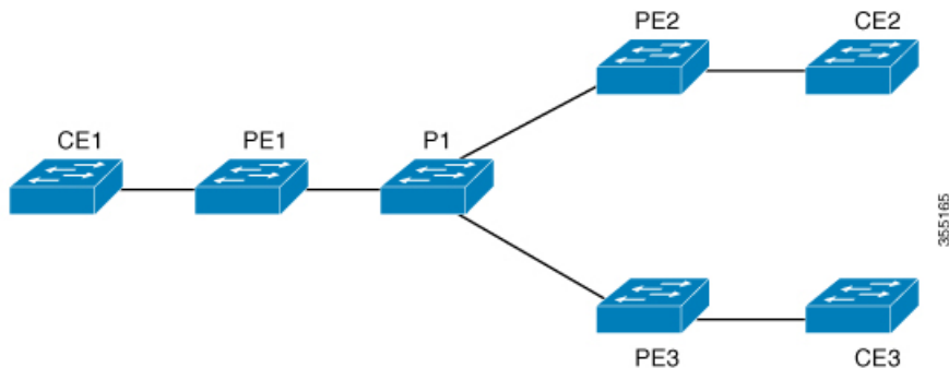
Figure 9: VPLS Topology
