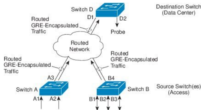
Figure 8: ERSPAN Configuration
