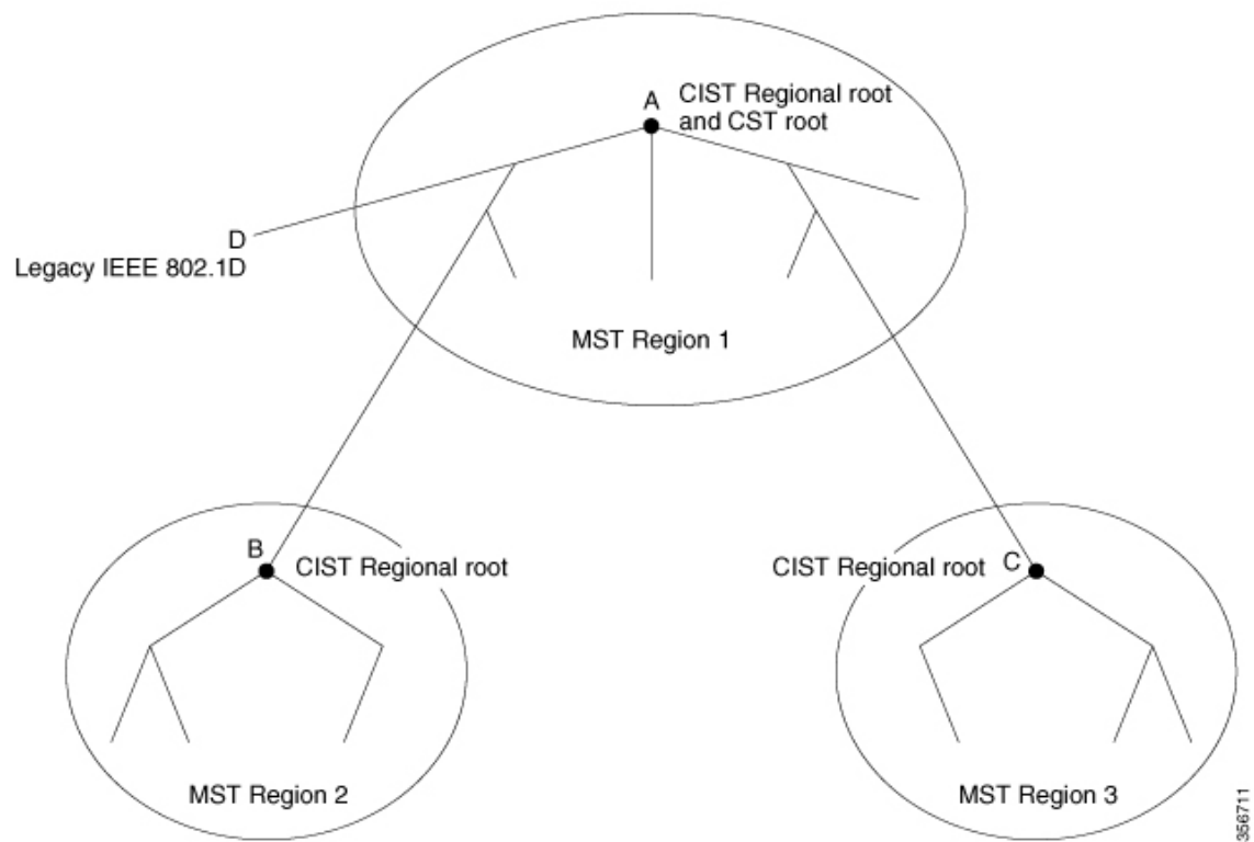
Figure 4: MST Regions, CIST Regional Root, and CIST Root
