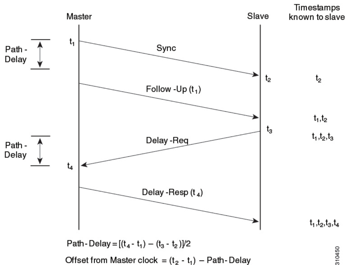
Figure 26: End-to-End Delay Mechanism
