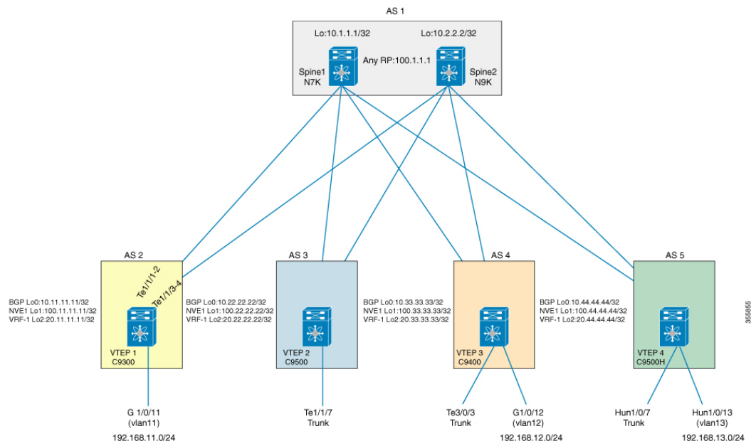
Figure 36: shows the topology used in the eBGP Multi-AS design model
