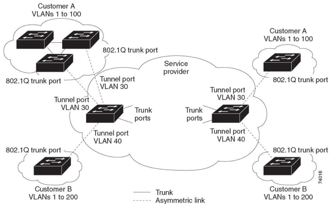
Figure 33: IEEE 802.1Q Tunnel Ports in a Service-Provider Network
