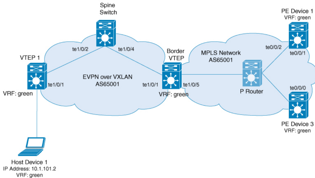
Figure 34: Layer 3 External Connectivity with MPLS Layer 3 VPN
