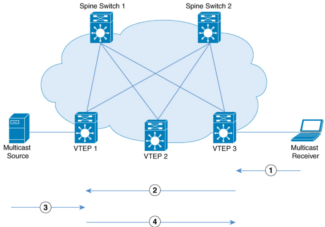
Figure 27: PIM Source Specific Mode
