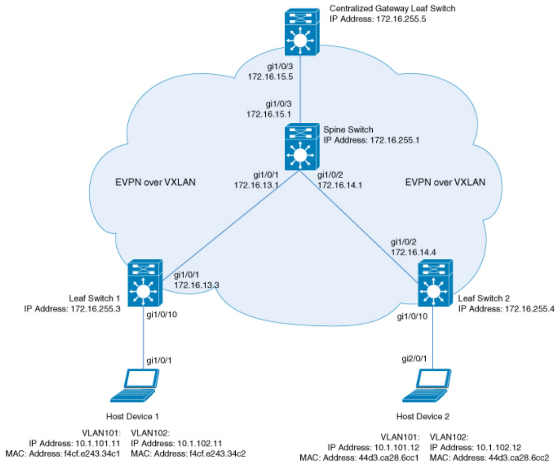
Figure 12: EVPN VXLAN Topology with Centralized Default Gateway
