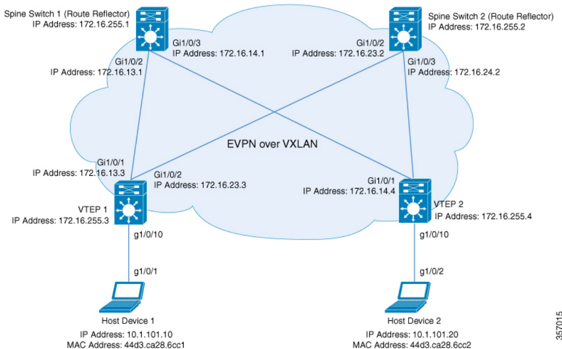
Figure 8: EVPN VXLAN Network with a Layer 2 VNI with Ingress Replication
