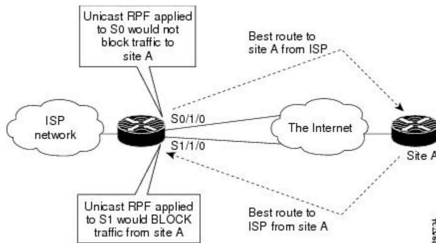
Figure 23: Unicast RPF Blocking Legitimate Traffic in an Asymmetric Routing Environment
