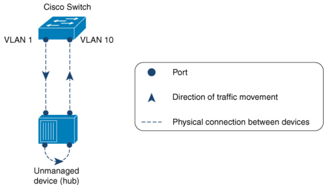
Figure 1: A Switch Connected to an Unmanaged Network Hub
