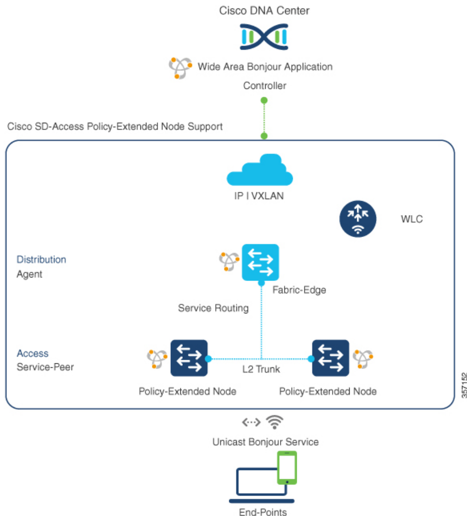
Figure 42: Fabric-Enabled Policy Extended Node
