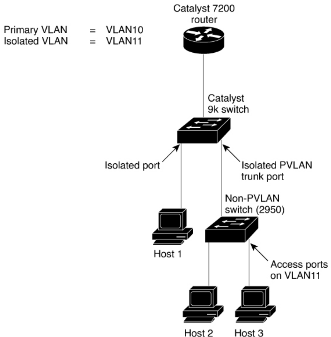
Figure 3: Isolated PVLAN Trunk Ports
