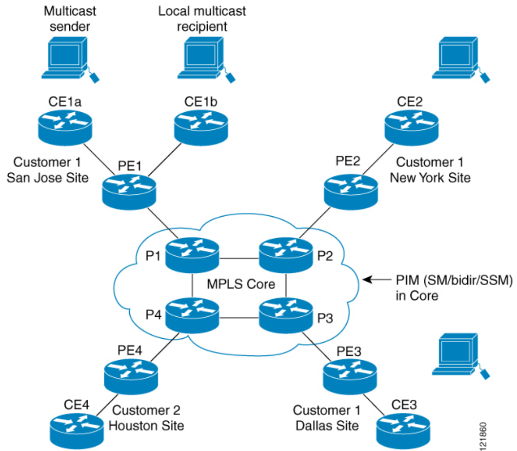
Figure 23: Default Multicast Distribution Tree Overview
