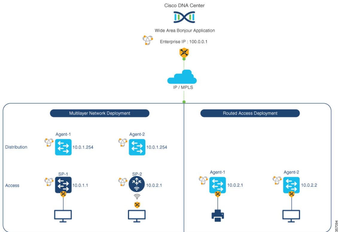
Figure 18: Cisco Wide Area Bonjour Configuration
