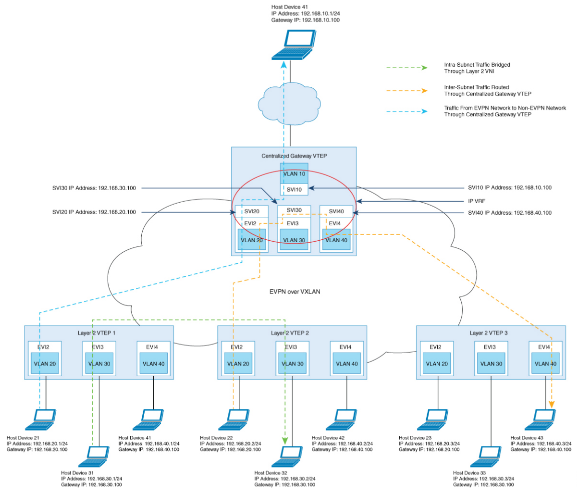
Figure 6: An EVPN VXLAN Network with Centralized Default Gateway
