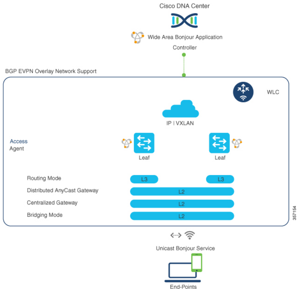
Figure 43: Overlay Bonjour Service for a BGP EVPN-Enabled Enterprise Network
