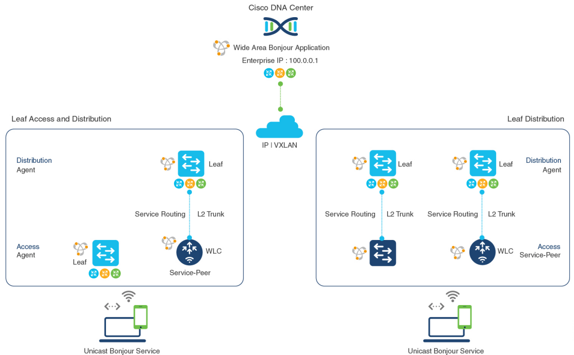
Figure 51: Deployment Model for Wide Area Bonjour over BGP EVPN VXLAN
