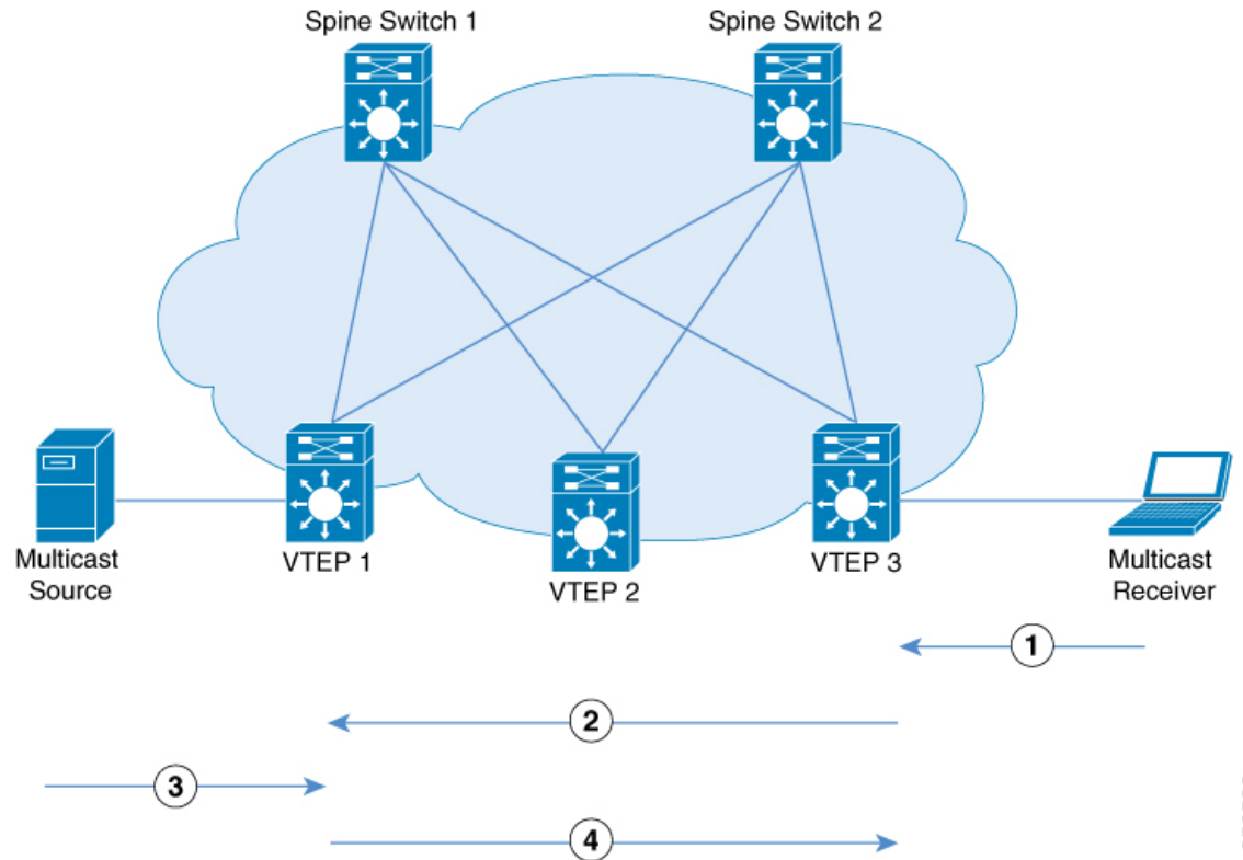
Figure 22: PIM Source Specific Mode
