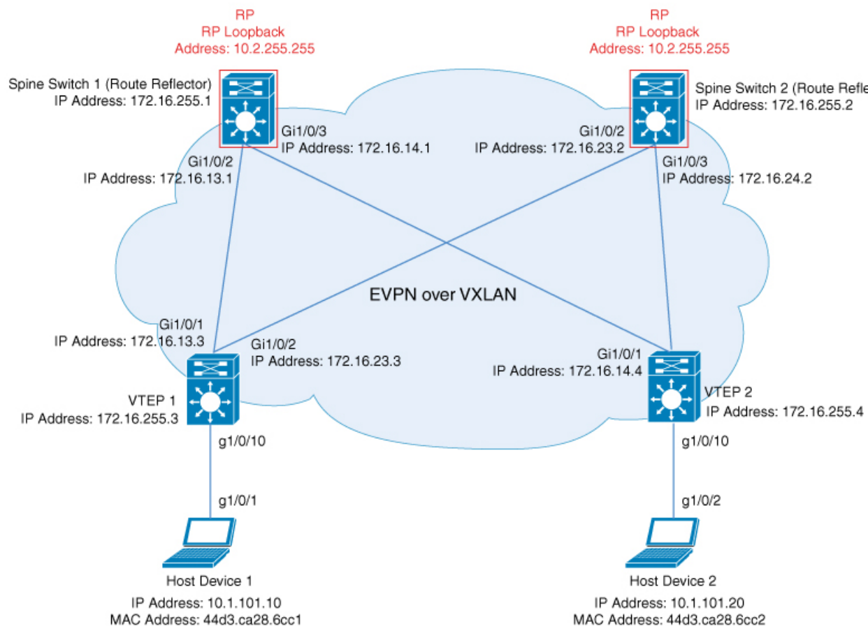
Figure 3: EVPN VXLAN Network with a Layer 2 VNI with Multicast Replication
