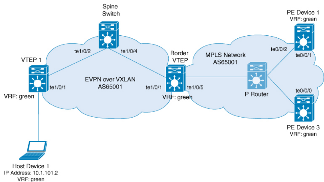
Figure 31: Layer 3 External Connectivity with MPLS Layer 3 VPN through iBGP
