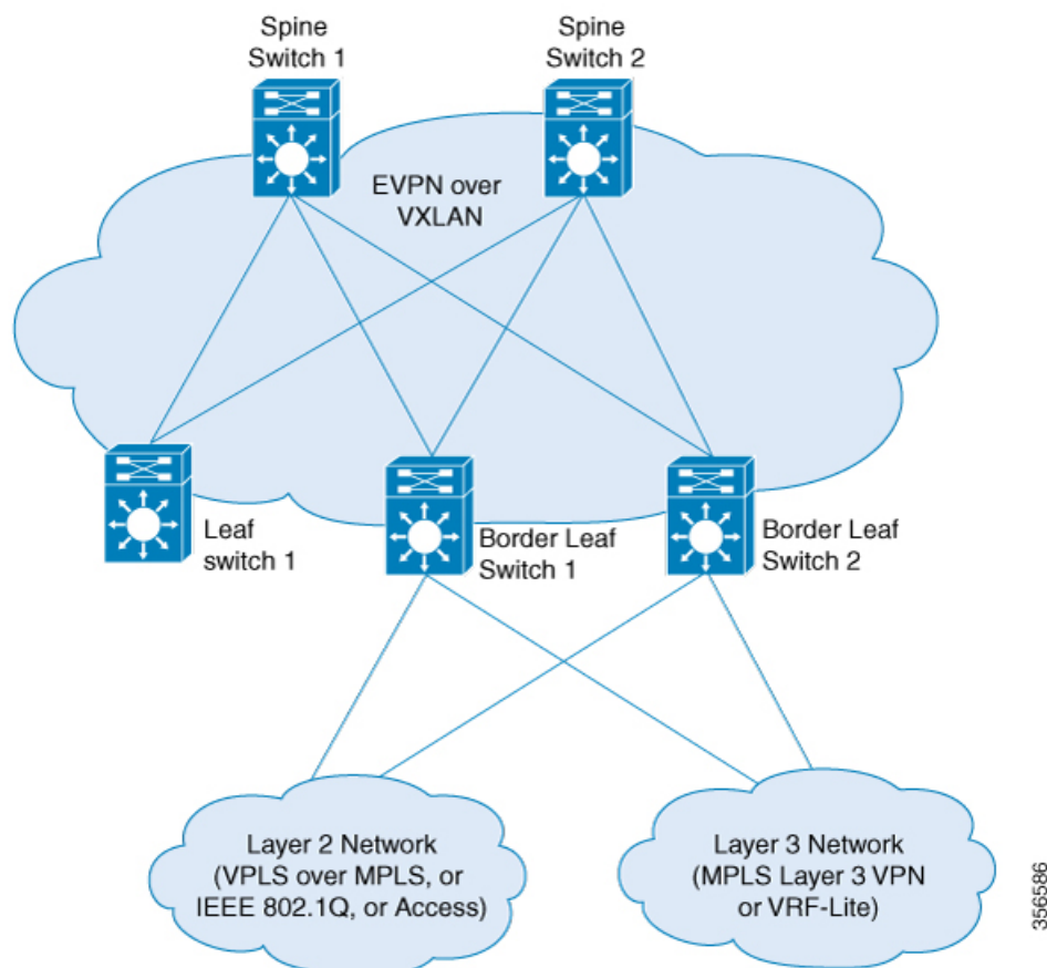
Figure 25: EVPN VXLAN External Connectivity Through a Border Leaf Switch
