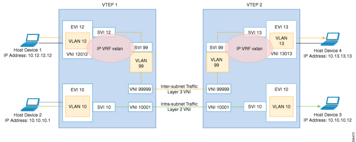
Figure 36: Movement of traffic in an EVPN VXLAN network through Layer2 and Layer 3 VNIs
