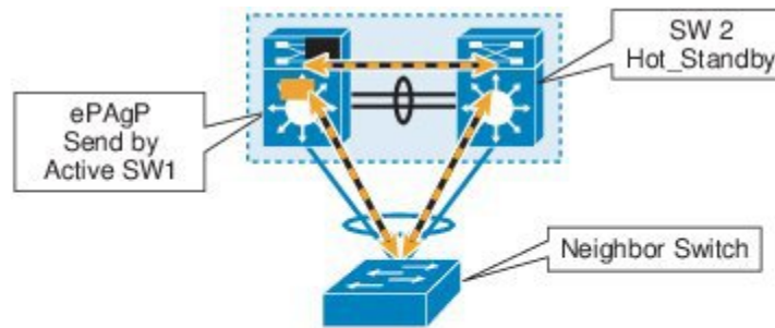
Figure 3: Dual-active-detection with ePAgP
