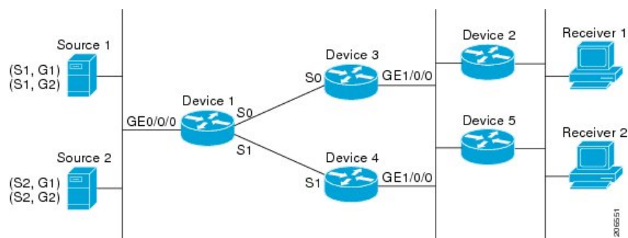
Figure 45: ECMP Multicast Load Splitting and the PIM Assert Process in PIM-SM and PIM-SSM
